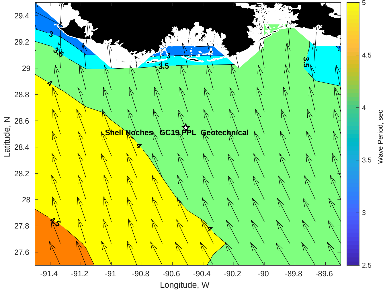
Wave Period (sec) for Shell Noches GC19 PPL Geotechnical at 25-May-2025 09:00:00
