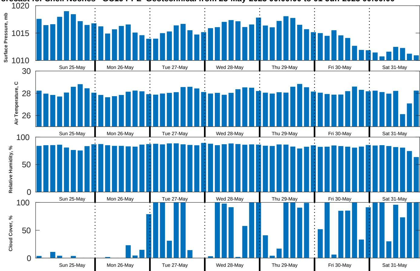
Met Forecast for Shell Noches GC19 PPL Geotechnical from 25-May-2025 00:00:00 to 01-Jun-2025 00:00:00
