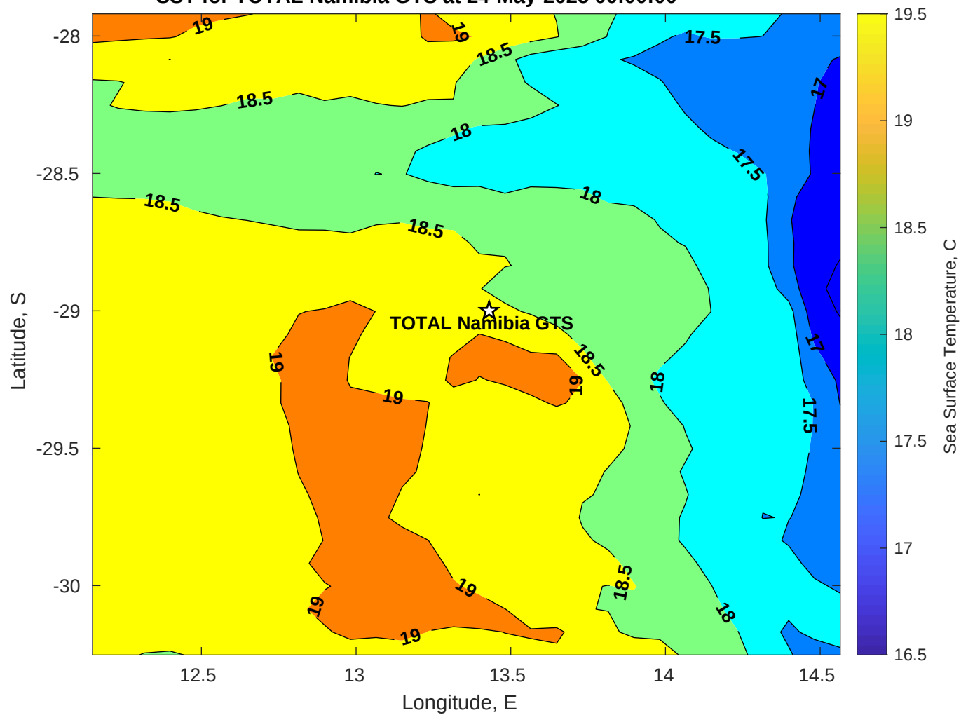
SST for TOTAL Namibia GTS at 24-May-2025 00:00:00
