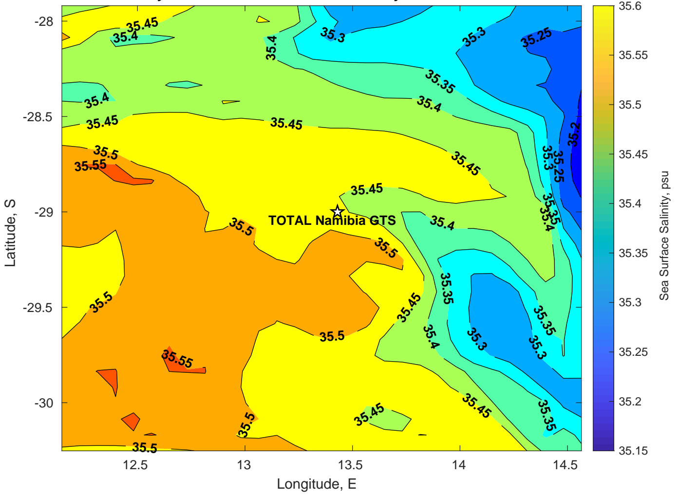
Surface Salinity for TOTAL Namibia GTS at 24-May-2025 00:00:00
