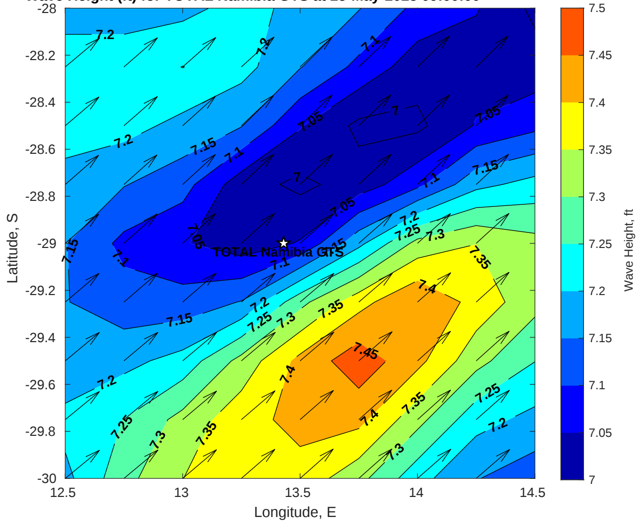
Wave Height (ft) for TOTAL Namibia GTS at 25-May-2025 09:00:00
