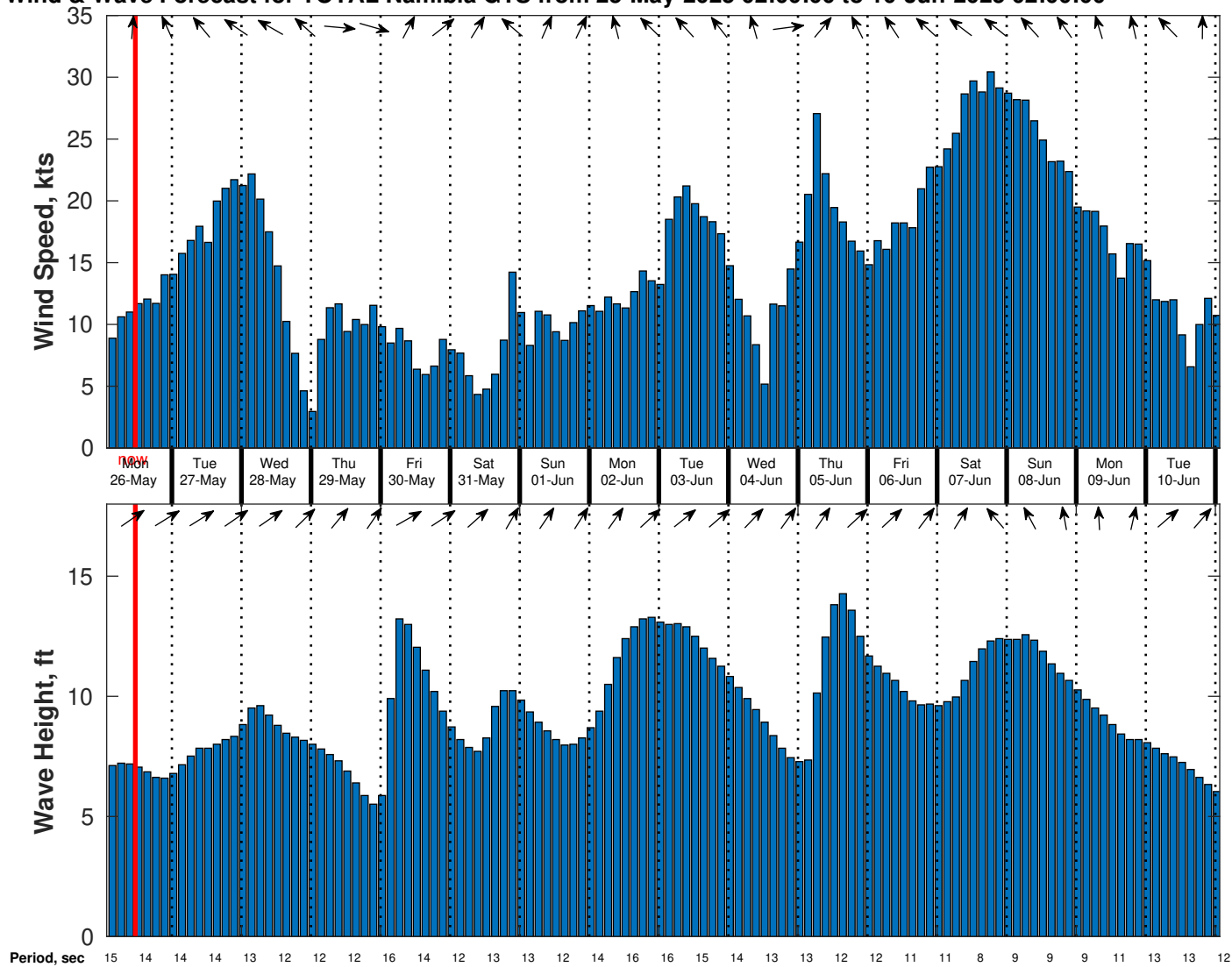
Wind & Wave Forecast for TOTAL Namibia GTS from 25-May-2025 02:00:00 to 10-Jun-2025 02:00:00
