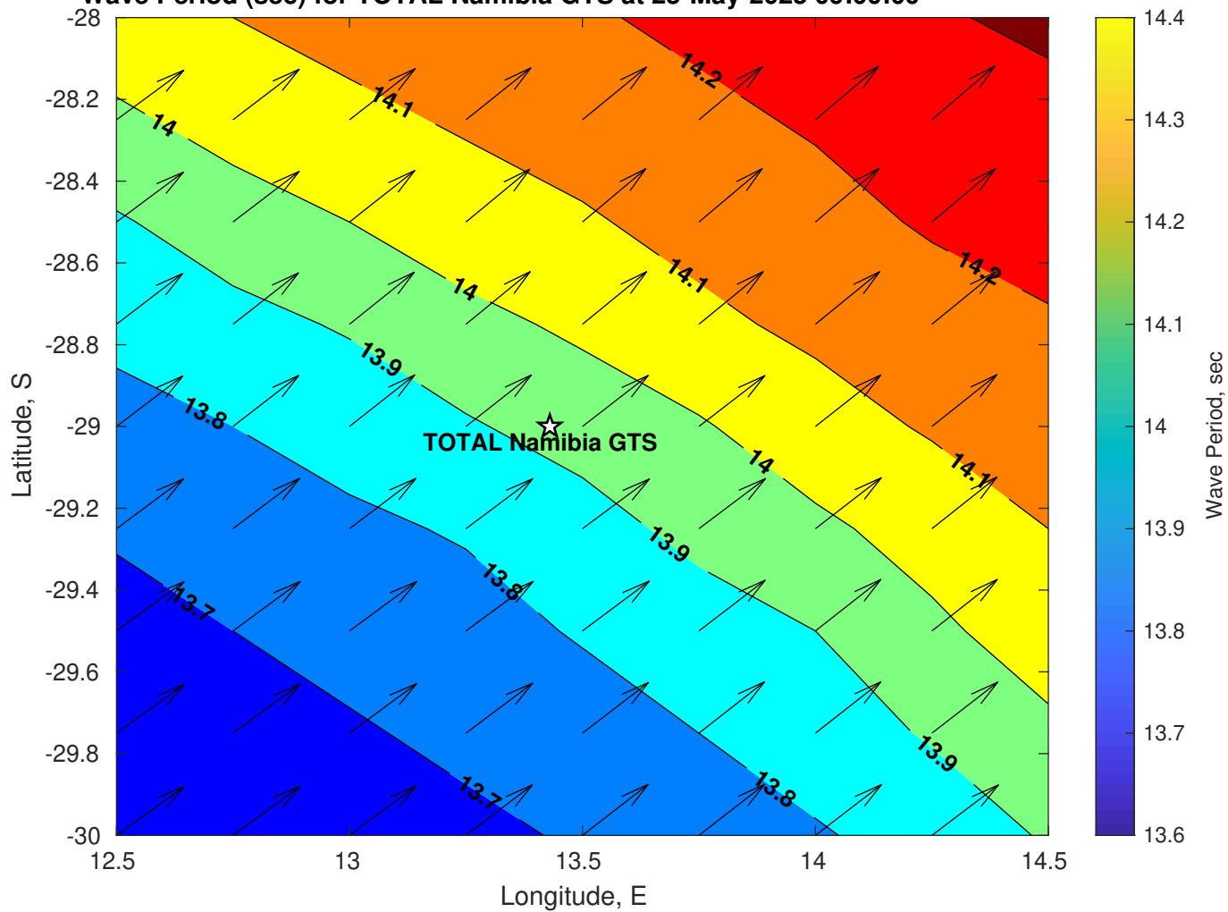
Wave Period (sec) for TOTAL Namibia GTS at 25-May-2025 09:00:00
