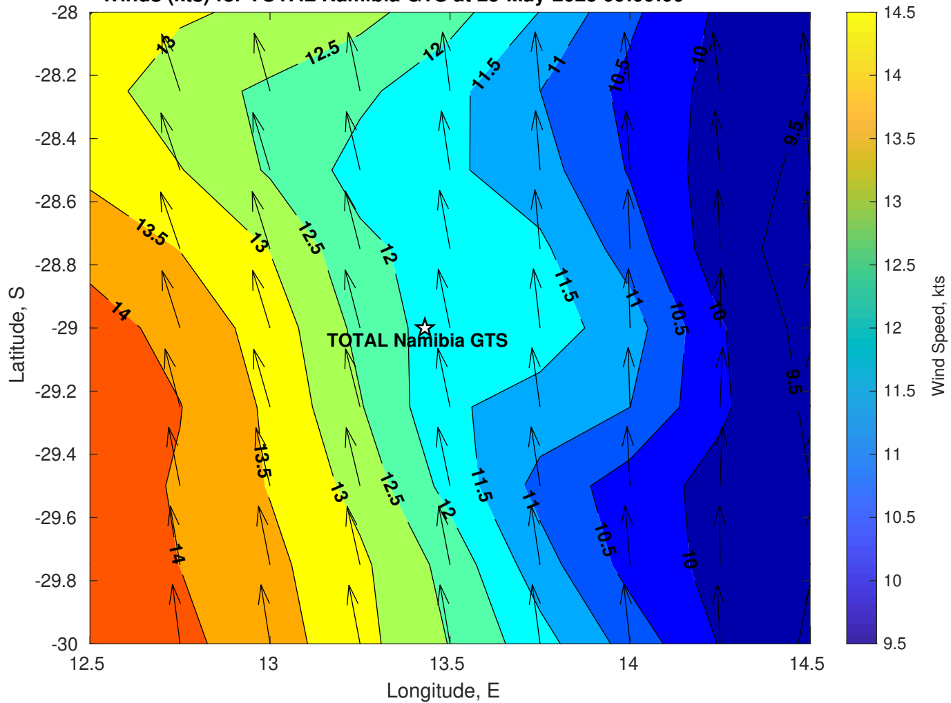
Winds (kts) for TOTAL Namibia GTS at 25-May-2025 09:00:00
