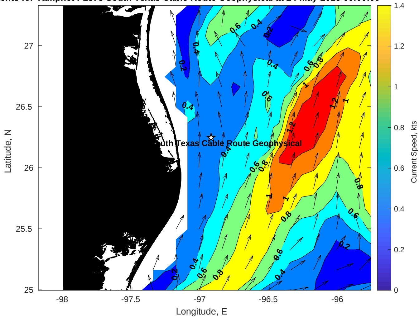
Surface Currents for Tampnet P2378 South Texas Cable Route Geophysical at 24-May-2025 00:00:00
