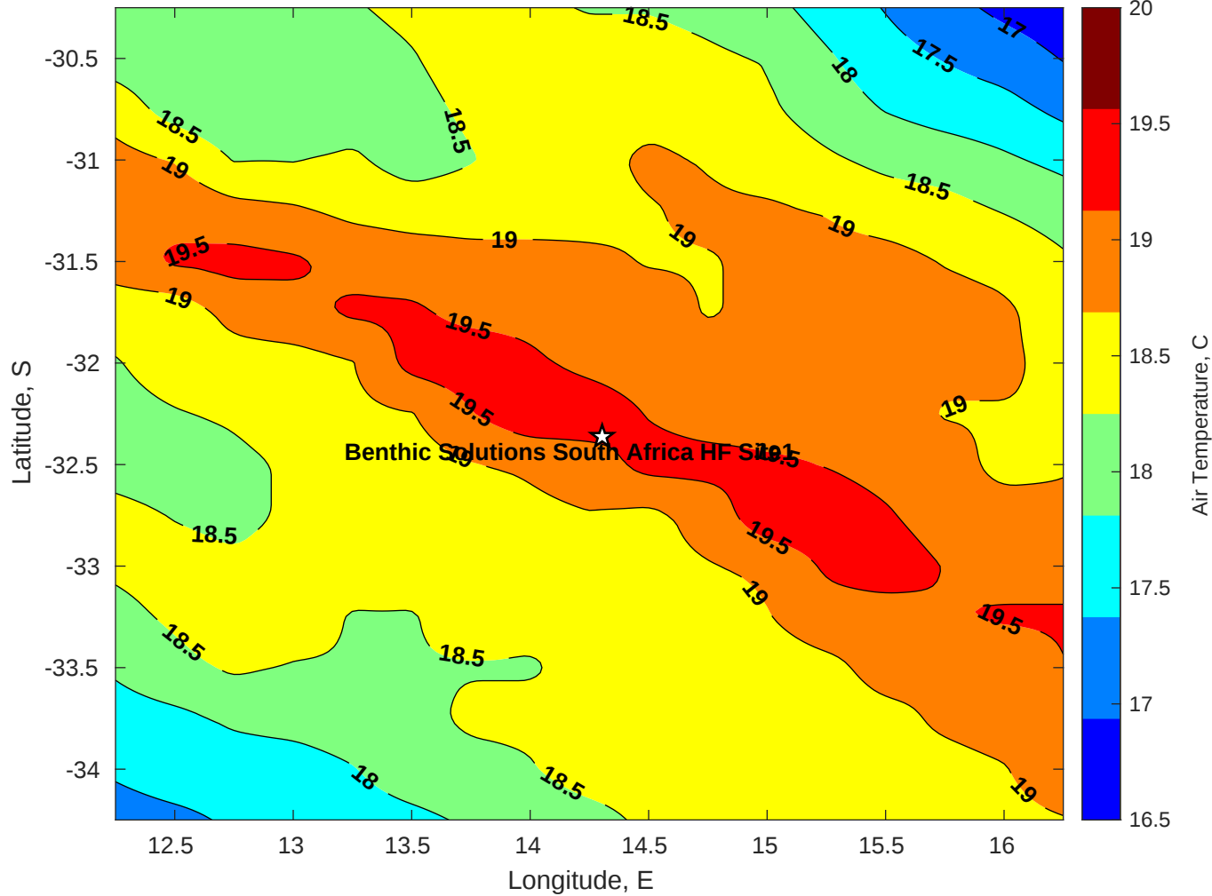
Air Temperature (C) for Benthic Solutions South Africa HF Site1 at 26-May-2025
