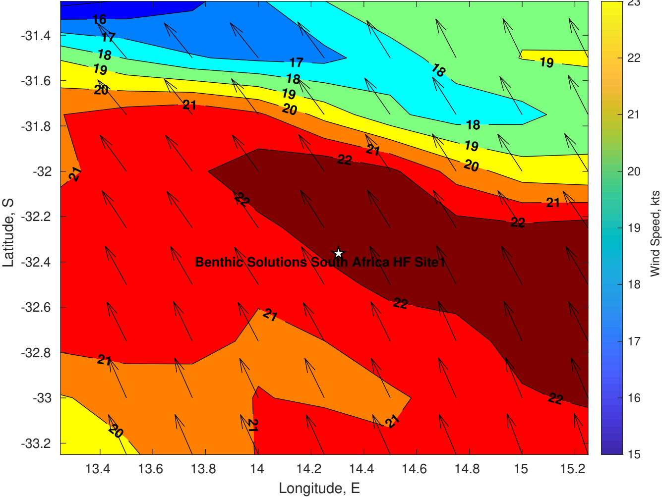
Winds (kts) for Benthic Solutions South Africa HF Site1 at 26-May-2025 09:00:00
