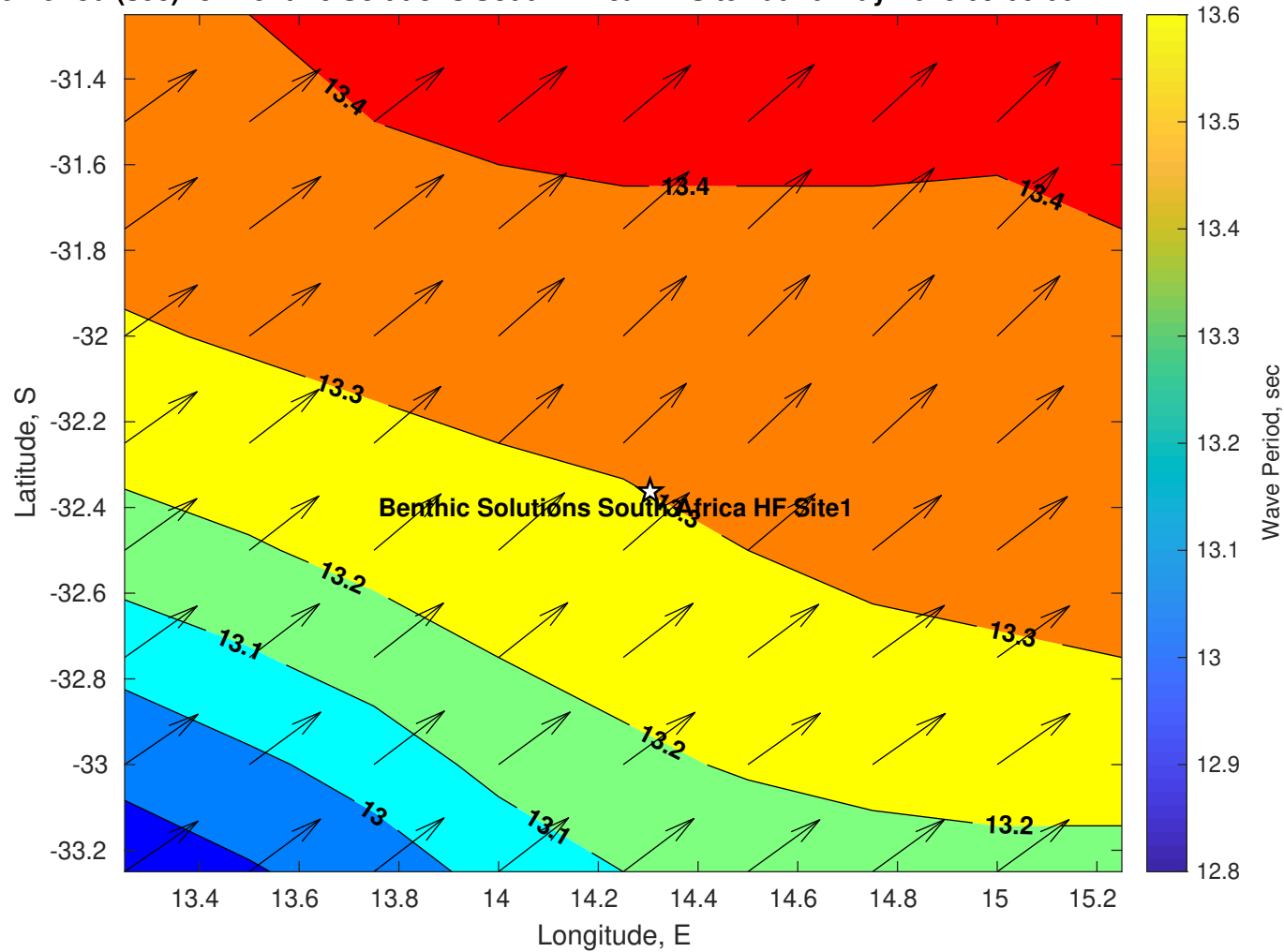
Wave Period (sec) for Benthic Solutions South Africa HF Site1 at 26-May-2025 09:00:00
