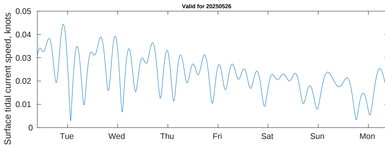
Tidal Currents and Heights for Benthic Solutions South Africa HF Site1 at 20250526
