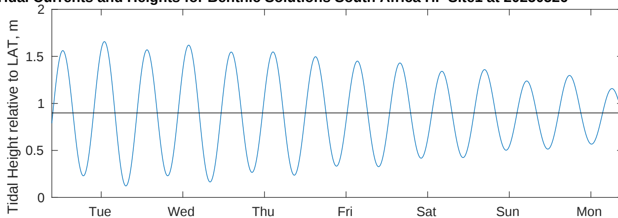
Tidal Currents and Heights for Benthic Solutions South Africa HF Site1 at 20250526
