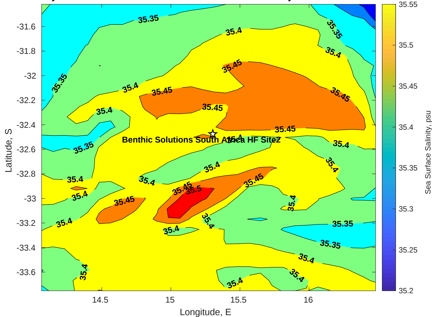
Surface Salinity for Benthic Solutions South Africa HF Site2 at 25-May-2025 00:00:00
