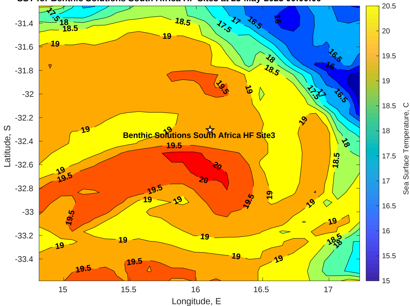
SST for Benthic Solutions South Africa HF Site3 at 25-May-2025 00:00:00
