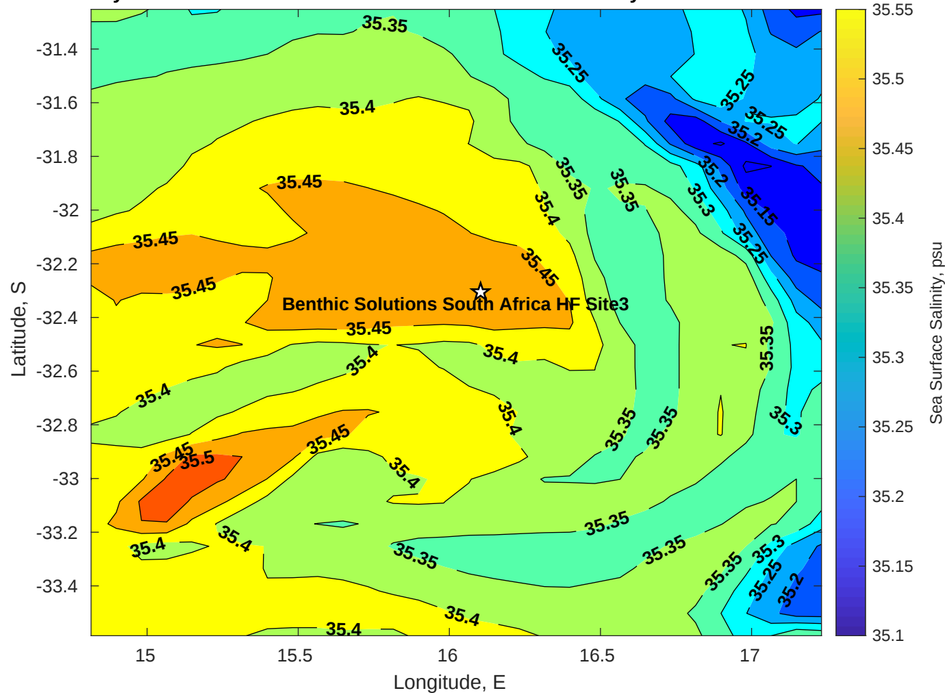
Surface Salinity for Benthic Solutions South Africa HF Site3 at 25-May-2025 00:00:00
