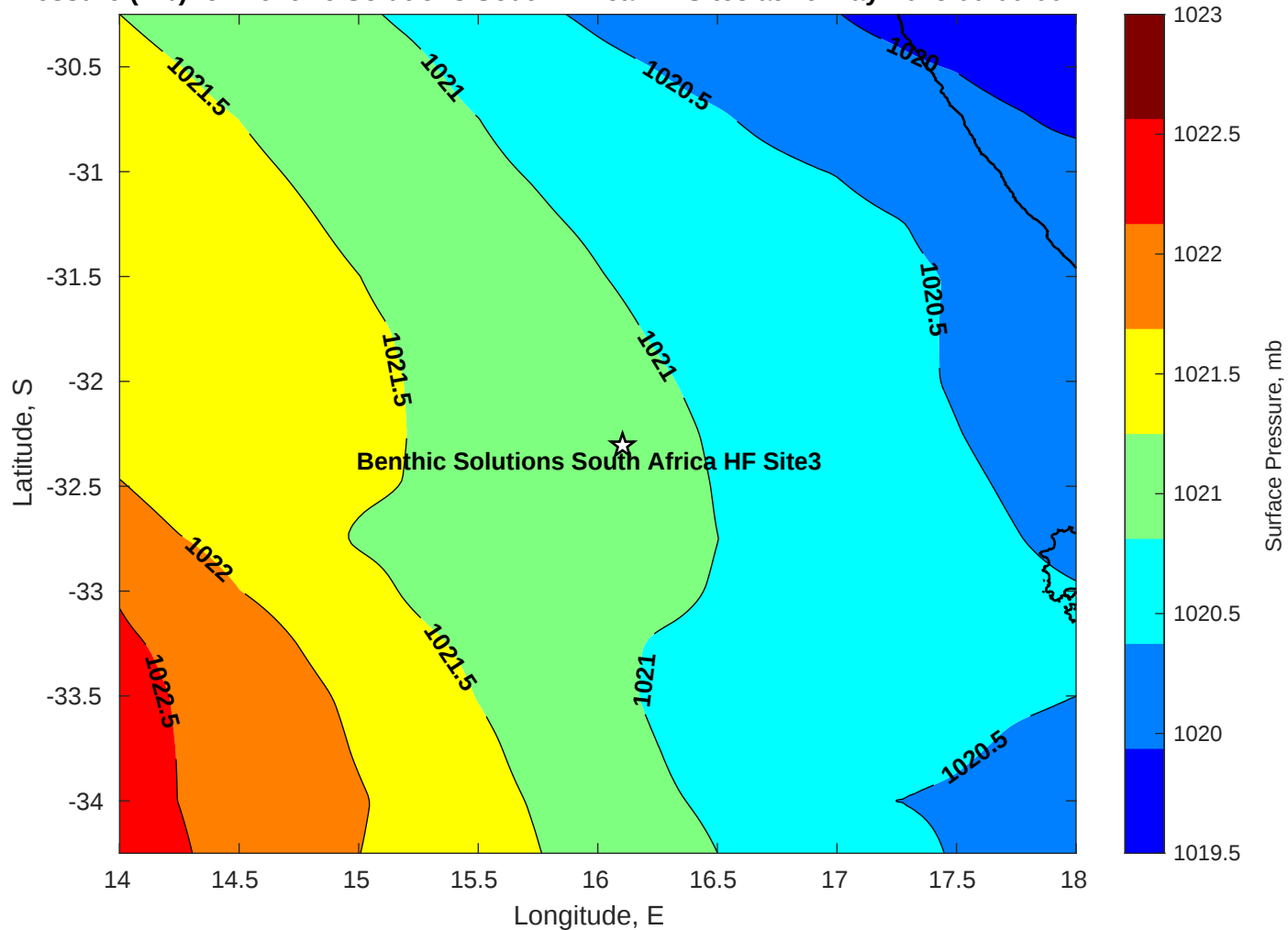
Surface Pressure (mb) for Benthic Solutions South Africa HF Site3 at 26-May-2025 00:00:00
