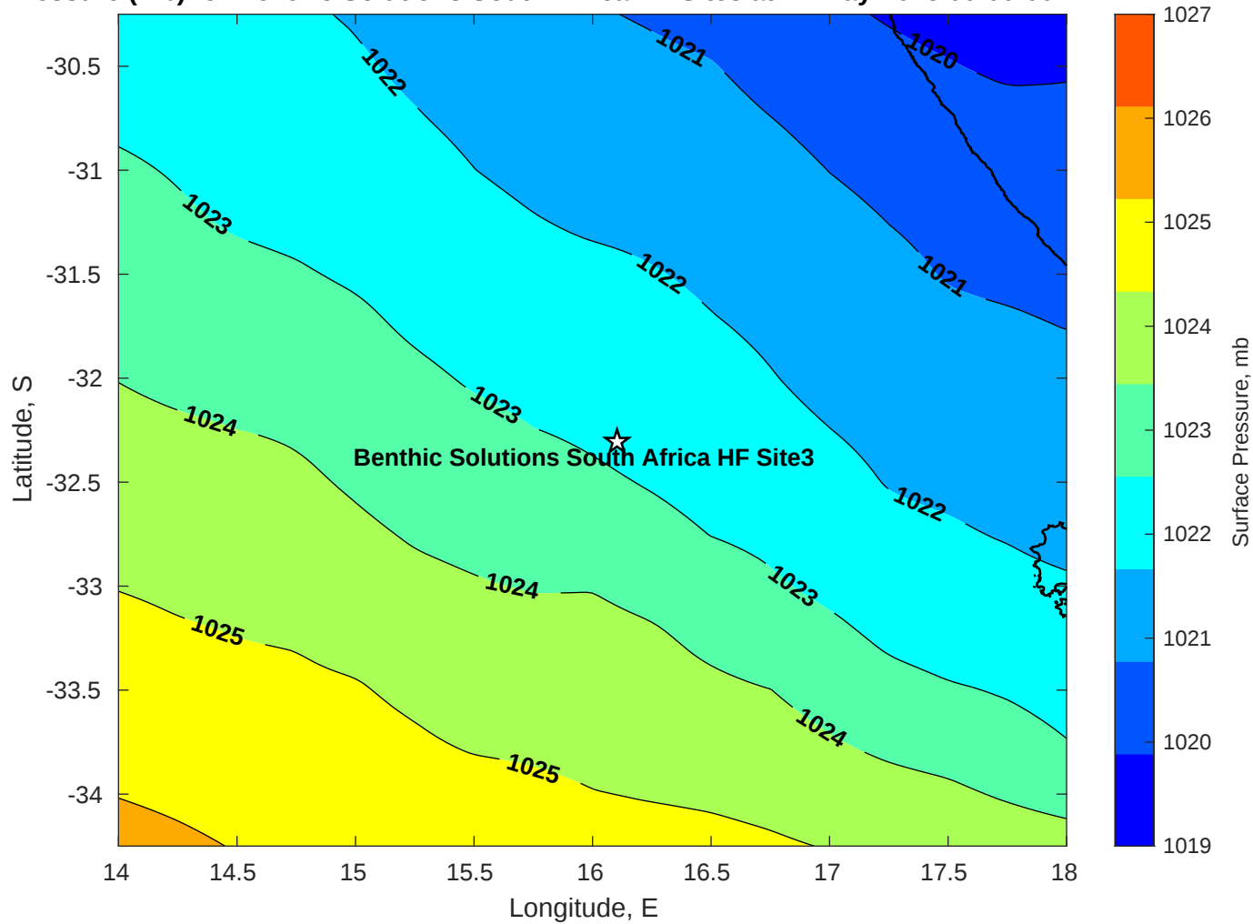
Surface Pressure (mb) for Benthic Solutions South Africa HF Site3 at 27-May-2025 00:00:00
