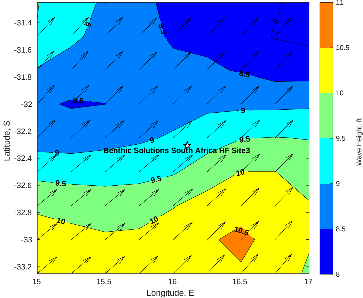
Wave Height (ft) for Benthic Solutions South Africa HF Site3 at 26-May-2025 09:00:00
