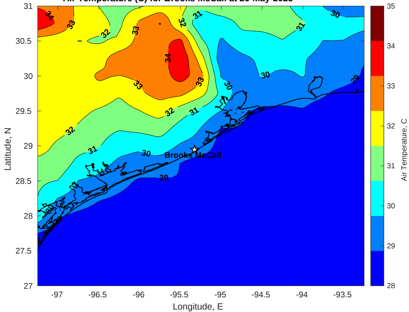
Air Temperature (C) for Brooks McCall at 26-May-2025
