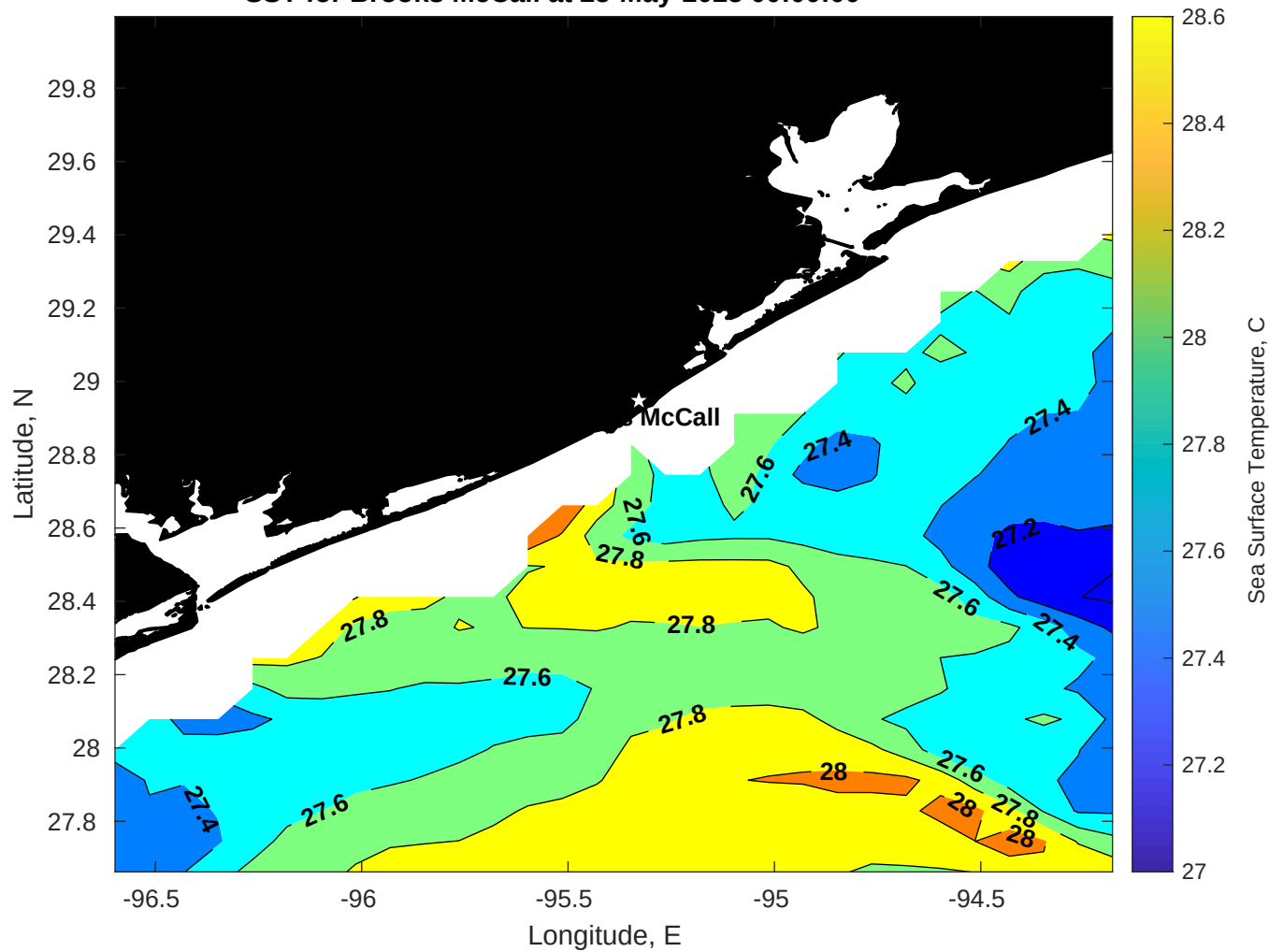
SST for Brooks McCall at 25-May-2025 00:00:00
