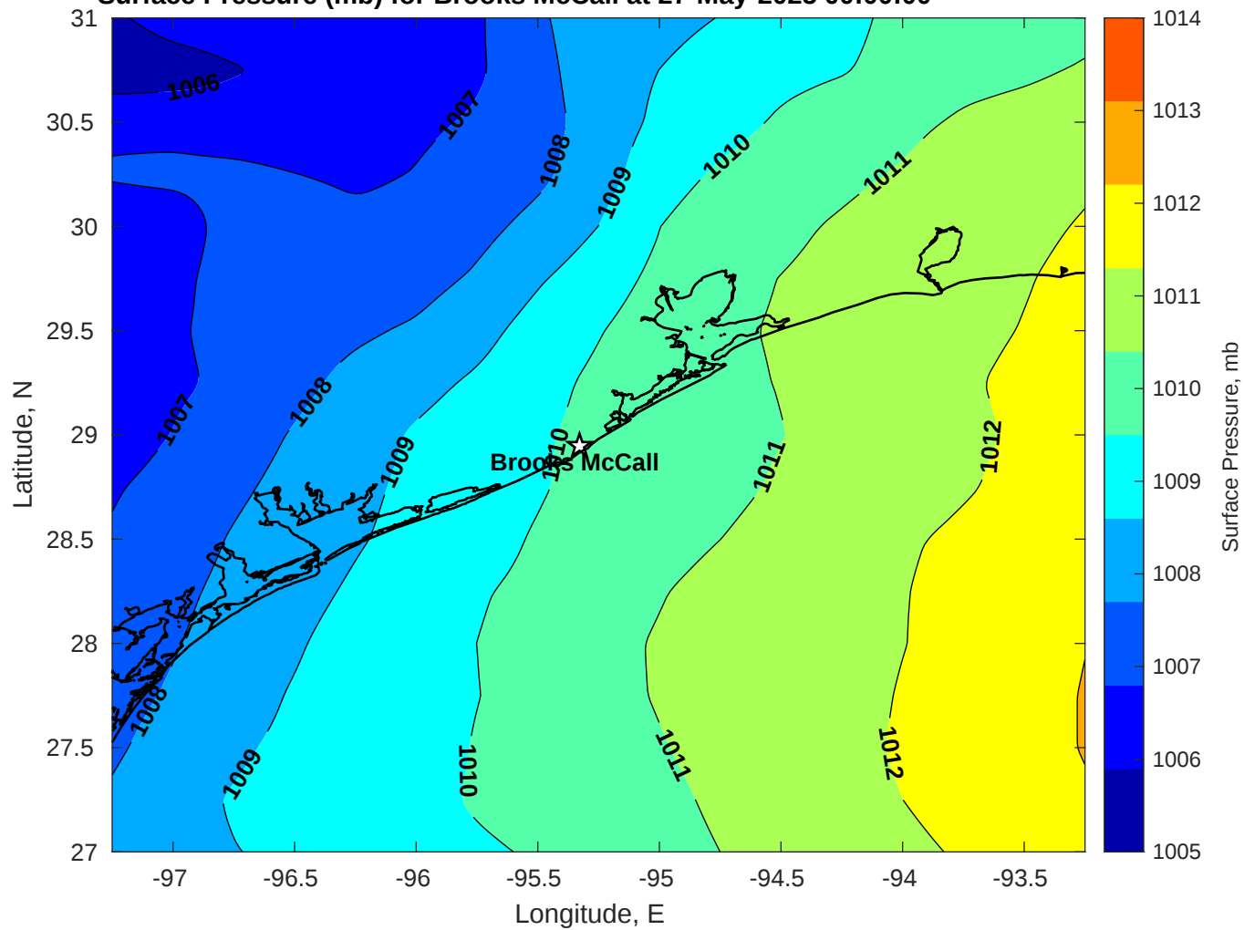
Surface Pressure (mb) for Brooks McCall at 27-May-2025 00:00:00
