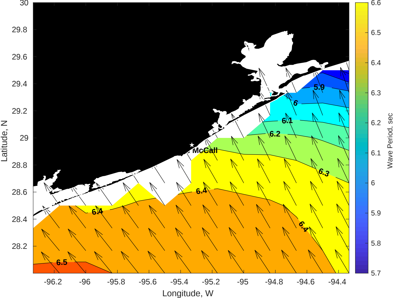
Wave Period (sec) for Brooks McCall at 26-May-2025 09:00:00
