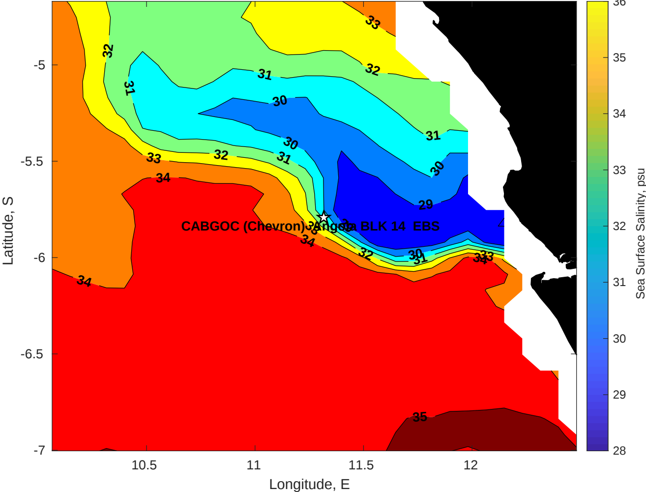
Surface Salinity for CABGOC (Chevron) Angola BLK 14 EBS at 25-May-2025 00:00:00
