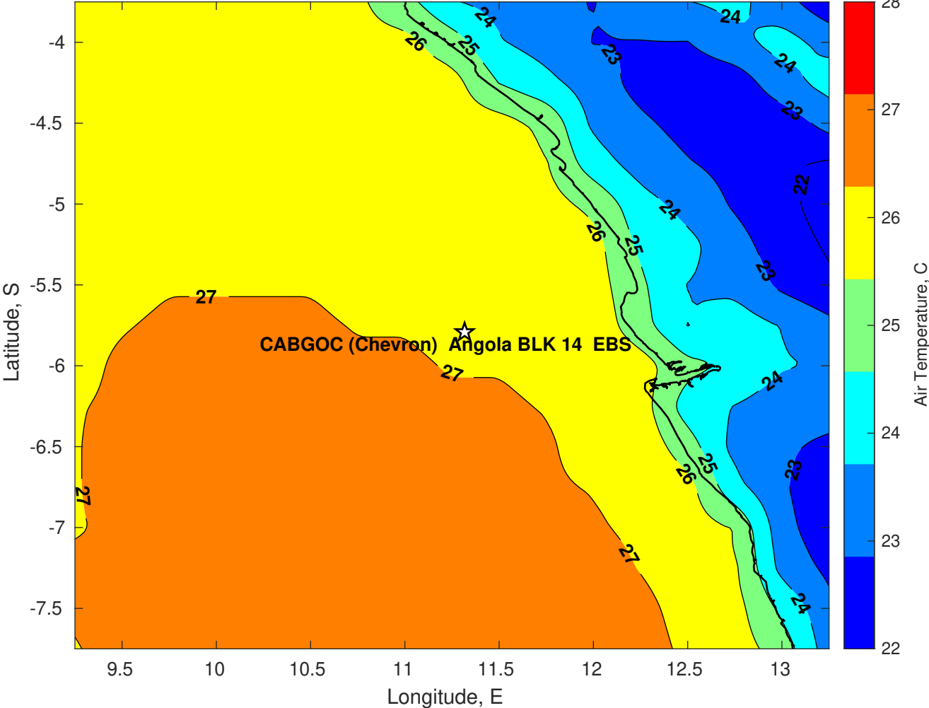
Air Temperature (C) for CABGOC (Chevron) Angola BLK 14 EBS at 26-May-2025
