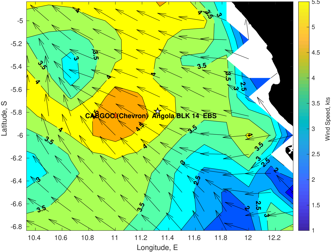
Winds (kts) for CABGOC (Chevron) Angola BLK 14 EBS at 26-May-2025 09:00:00
