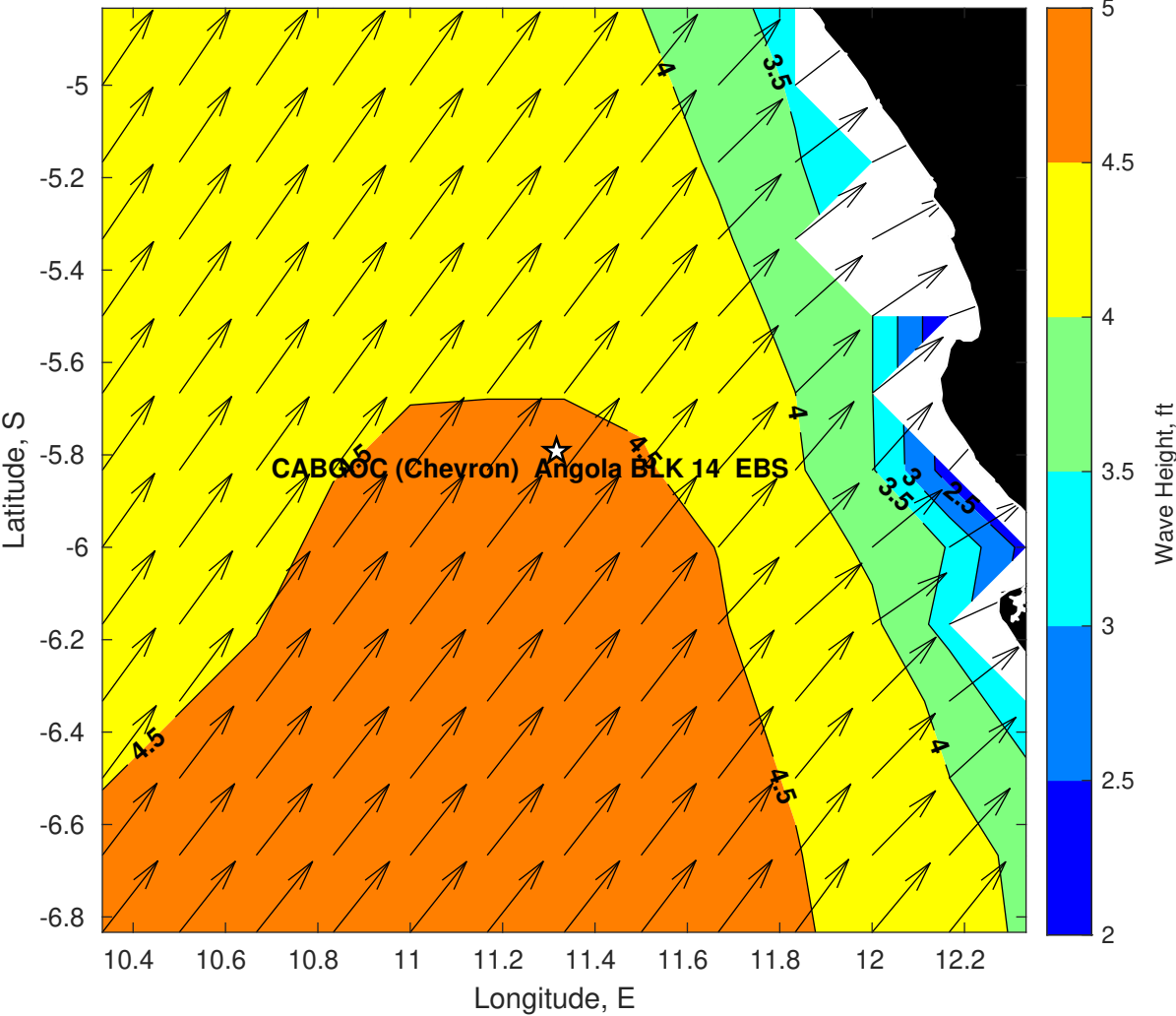
Wave Height (ft) for CABGOC (Chevron) Angola BLK 14 EBS at 26-May-2025 09:00:00
