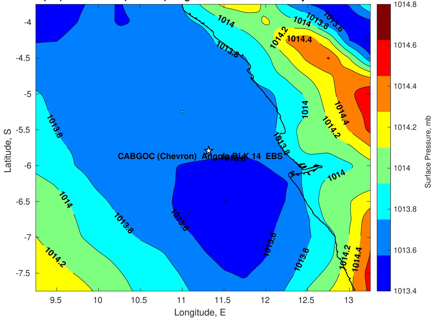
Surface Pressure (mb) for CABGOC (Chevron) Angola BLK 14 EBS at 28-May-2025 00:00:00
