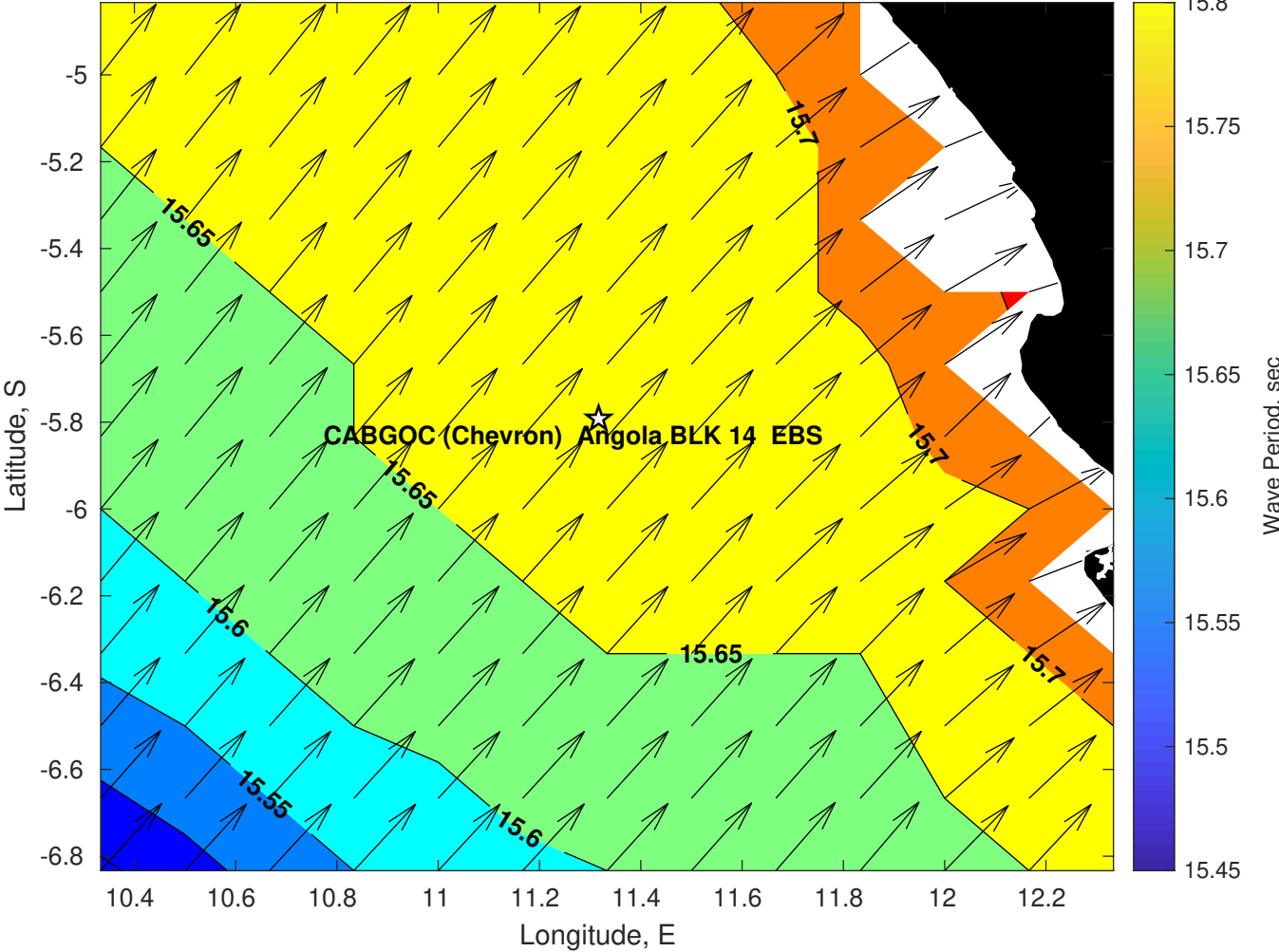
Wave Period (sec) for CABGOC (Chevron) Angola BLK 14 EBS at 26-May-2025 09:00:00
