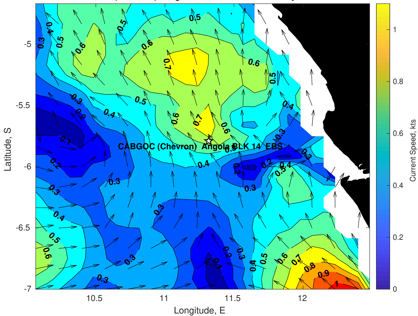
Surface Currents for CABGOC (Chevron) Angola BLK 14 EBS at 25-May-2025 00:00:00
