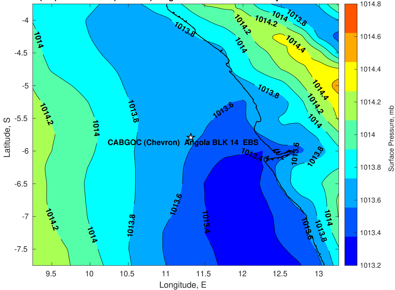
Surface Pressure (mb) for CABGOC (Chevron) Angola BLK 14 EBS at 27-May-2025 00:00:00
