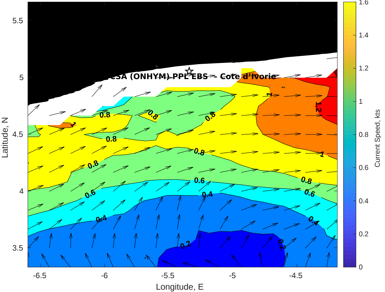
Surface Currents for CSA (ONHYM) PPL EBS - Cote d'Ivoire at 25-May-2025 00:00:00
