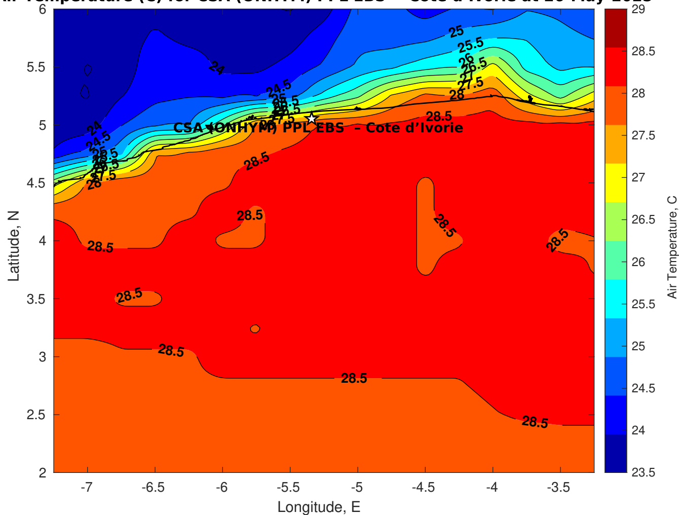
Air Temperature (C) for CSA (ONHYM) PPL EBS - Cote d'Ivoire at 26-May-2025
