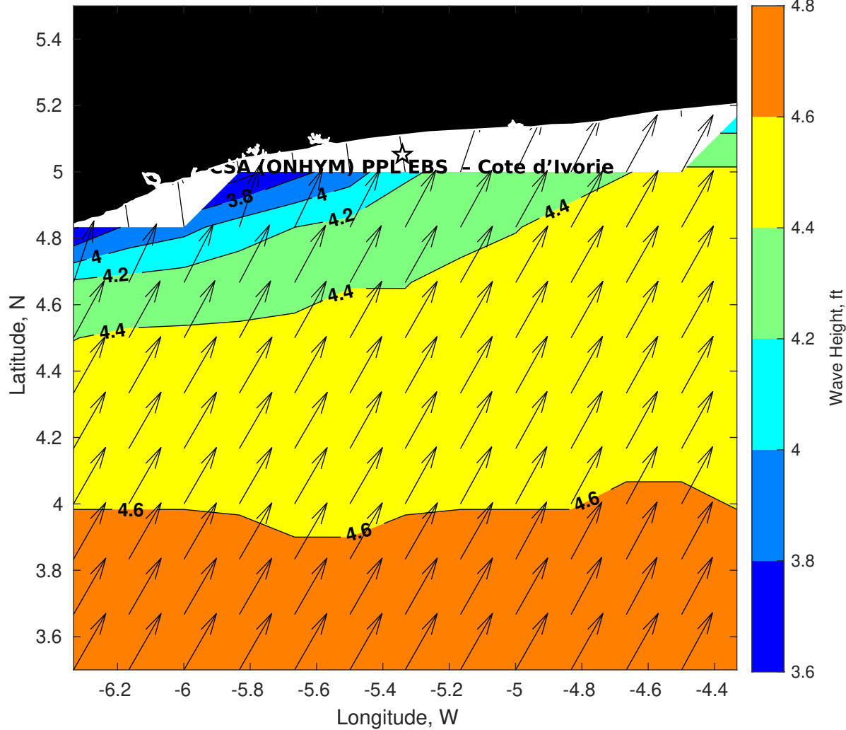
Wave Height (ft) for CSA (ONHYM) PPL EBS - Cote d'Ivoire at 26-May-2025 09:00:00
