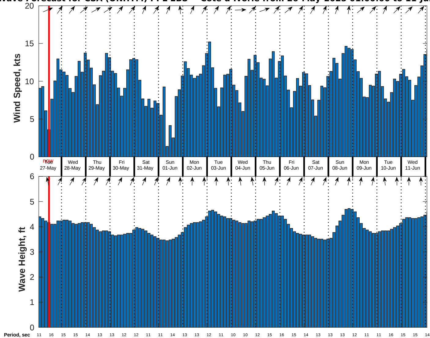
Wind & Wave Forecast for CSA (ONHYM) PPL EBS - Cote d'Ivoire from 26-May-2025 01:00:00 to 11-Jun-2025 01:00:00
