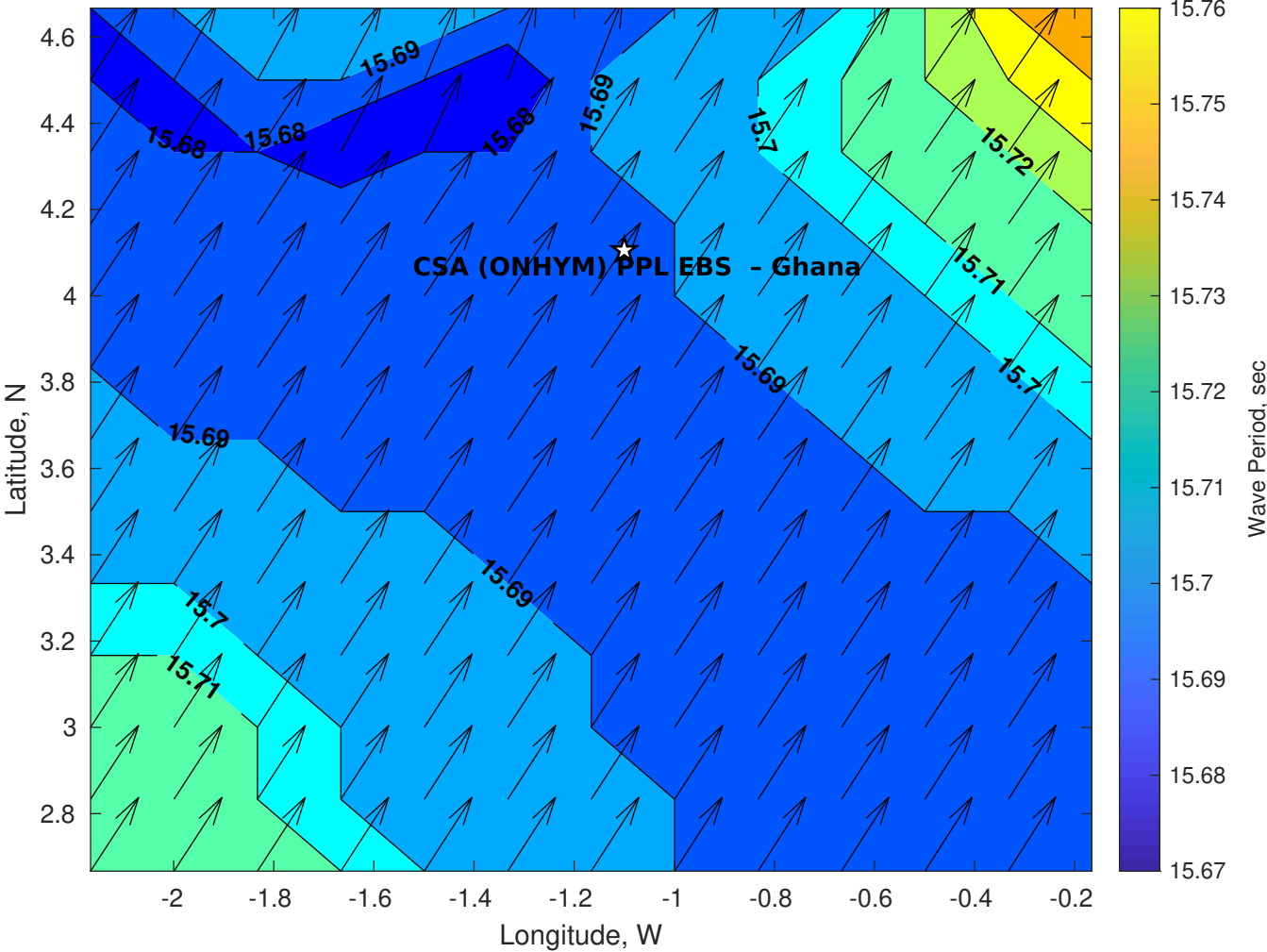
Wave Period (sec) for CSA (ONHYM) PPL EBS - Ghana at 26-May-2025 09:00:00
