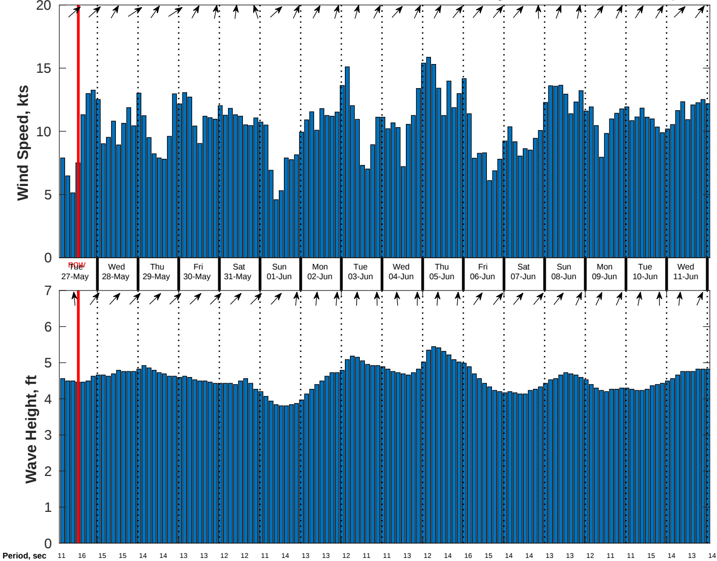
Wind & Wave Forecast for CSA (ONHYM) PPL EBS - Ghana from 26-May-2025 02:00:00 to 11-Jun-2025 02:00:00
