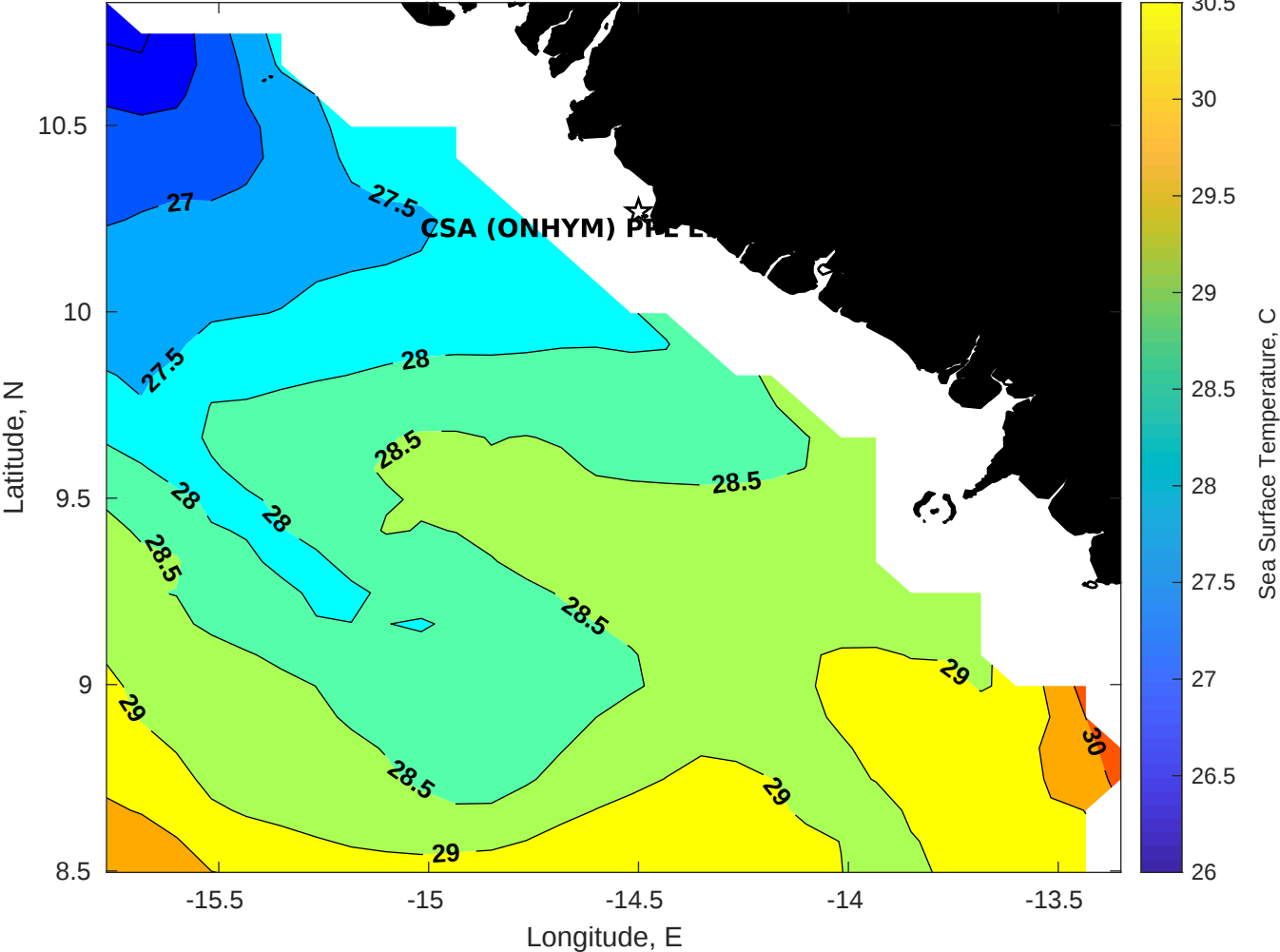
SST for CSA (ONHYM) PPL EBS - Guinea at 25-May-2025 00:00:00
