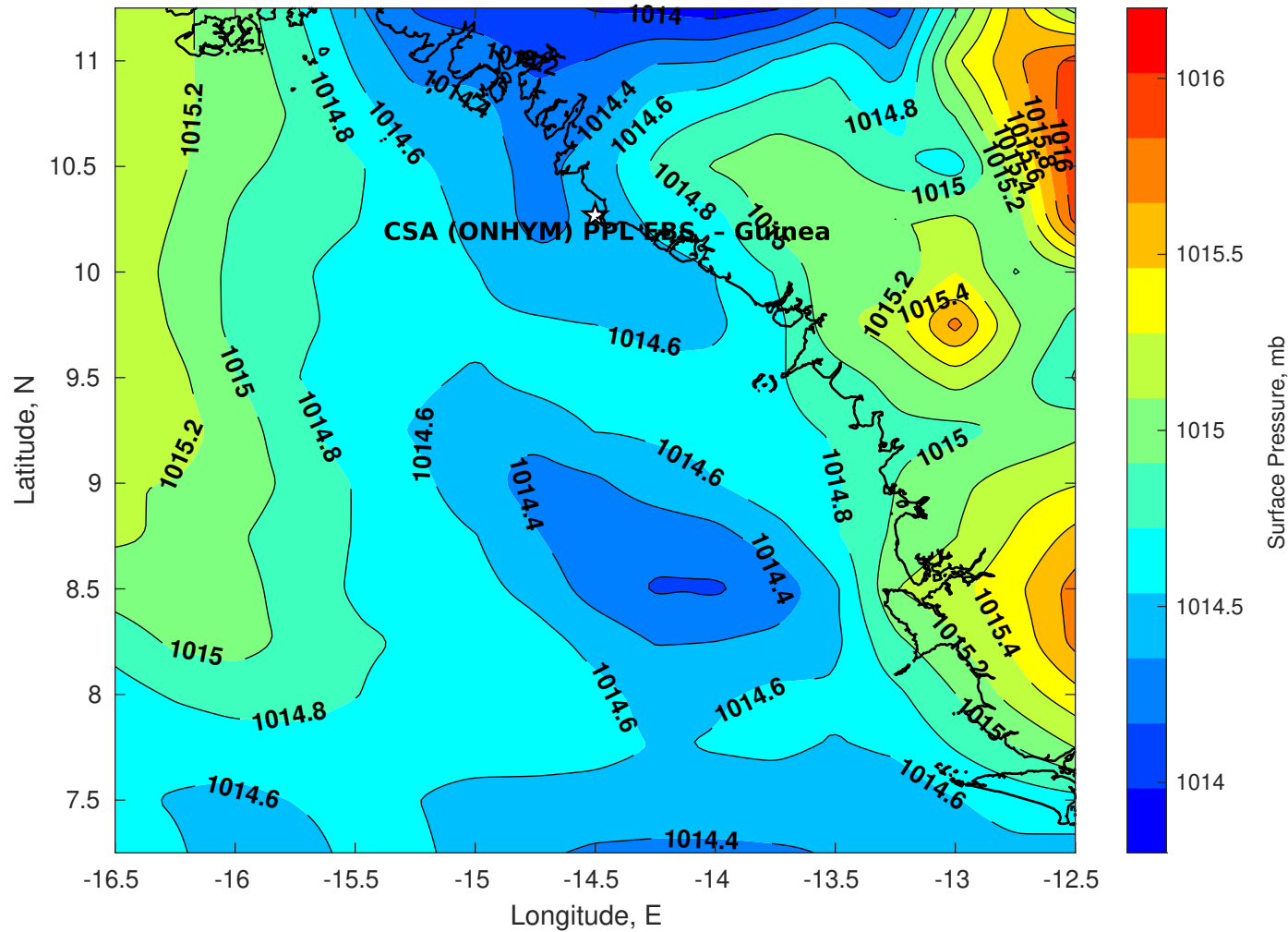
Surface Pressure (mb) for CSA (ONHYM) PPL EBS - Guinea at 28-May-2025 00:00:00
