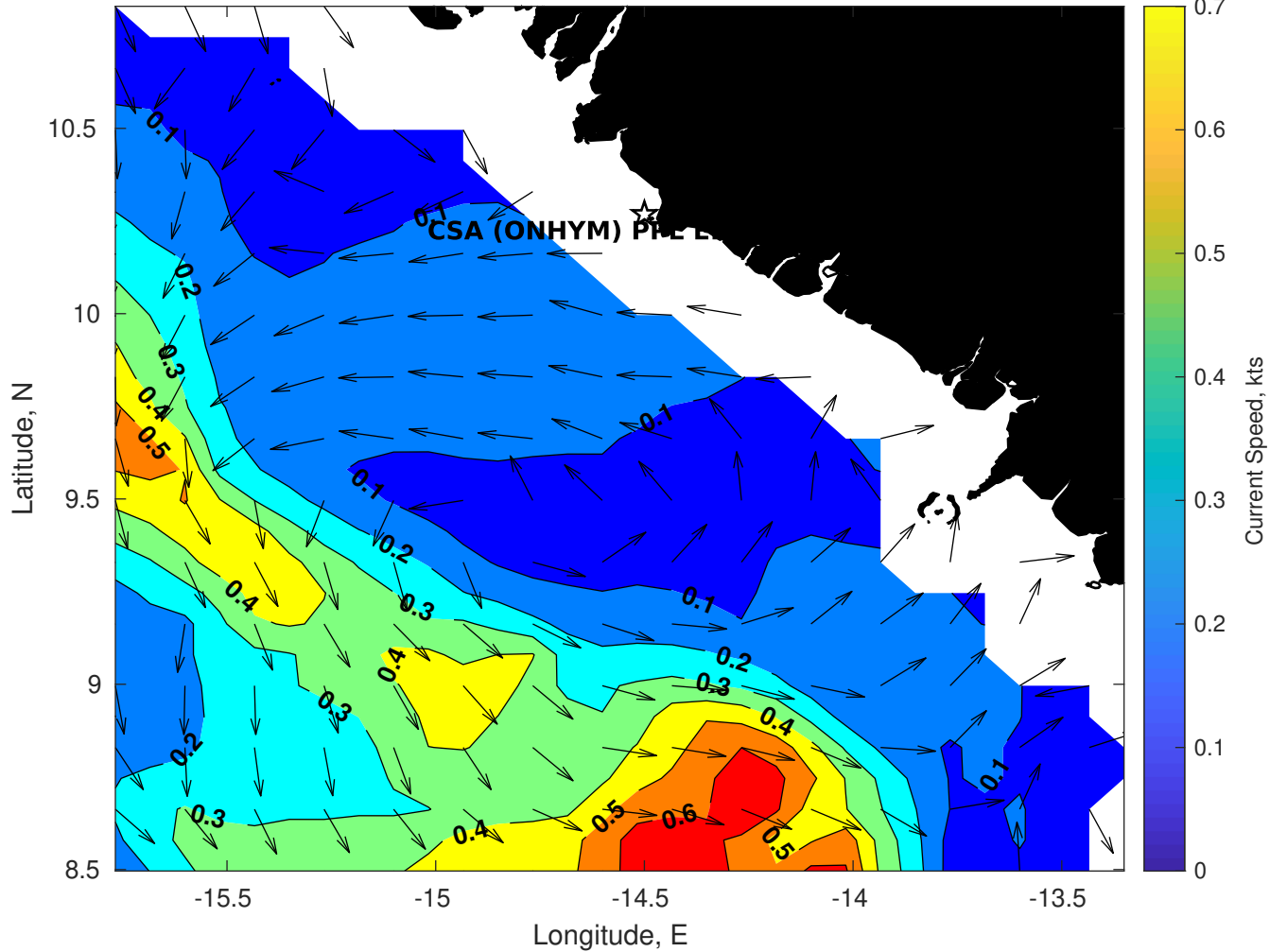
Surface Currents for CSA (ONHYM) PPL EBS - Guinea at 25-May-2025 00:00:00
