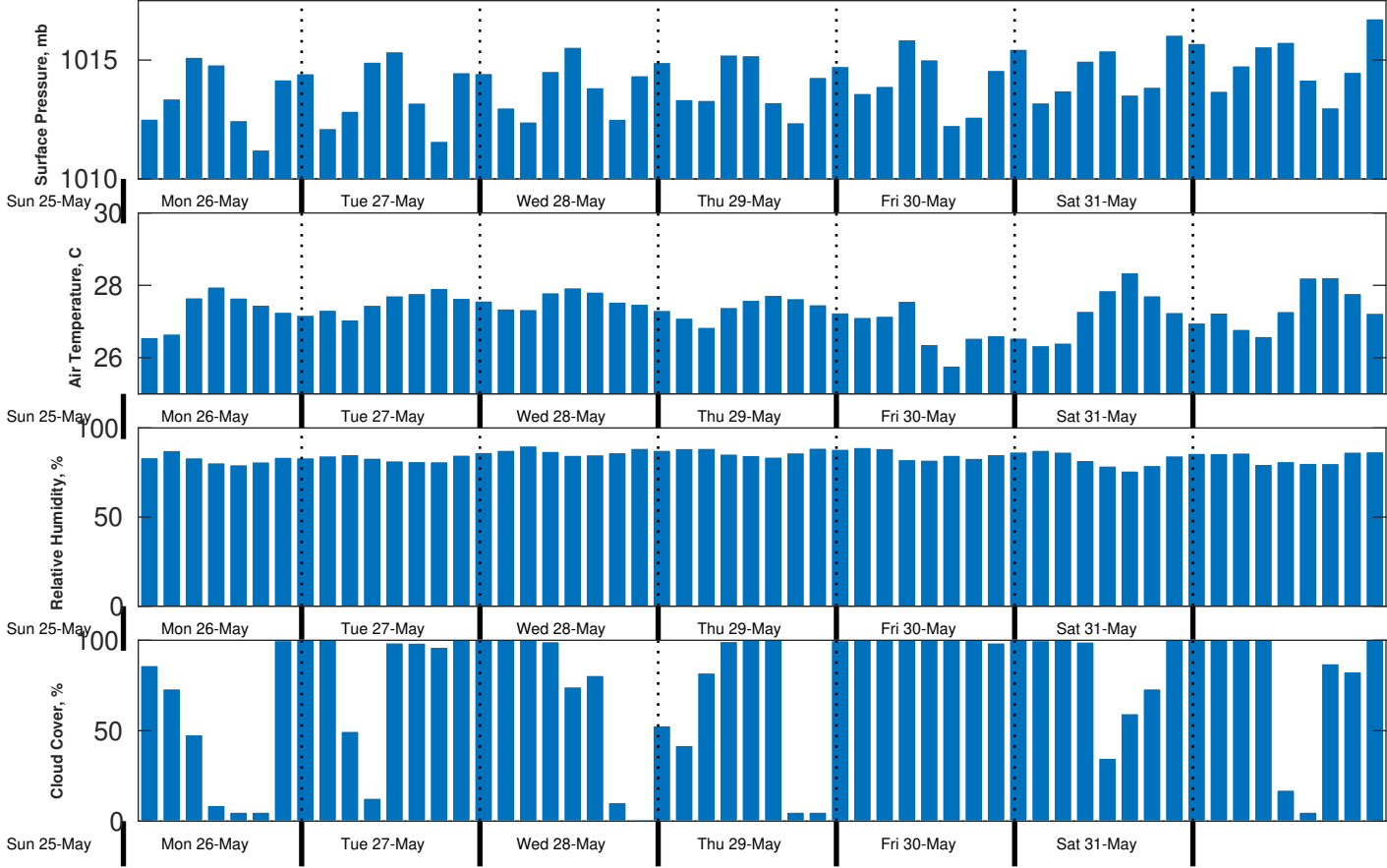
Met Forecast for CSA (ONHYM) PPL EBS - Guinea from 26-May-2025 00:00:00 to 02-Jun-2025 00:00:00
