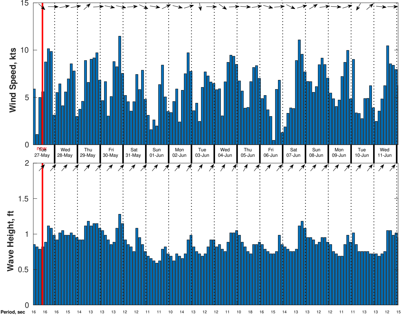
Wind & Wave Forecast for CSA (ONHYM) PPL EBS - Guinea from 26-May-2025 01:00:00 to 11-Jun-2025 01:00:00
