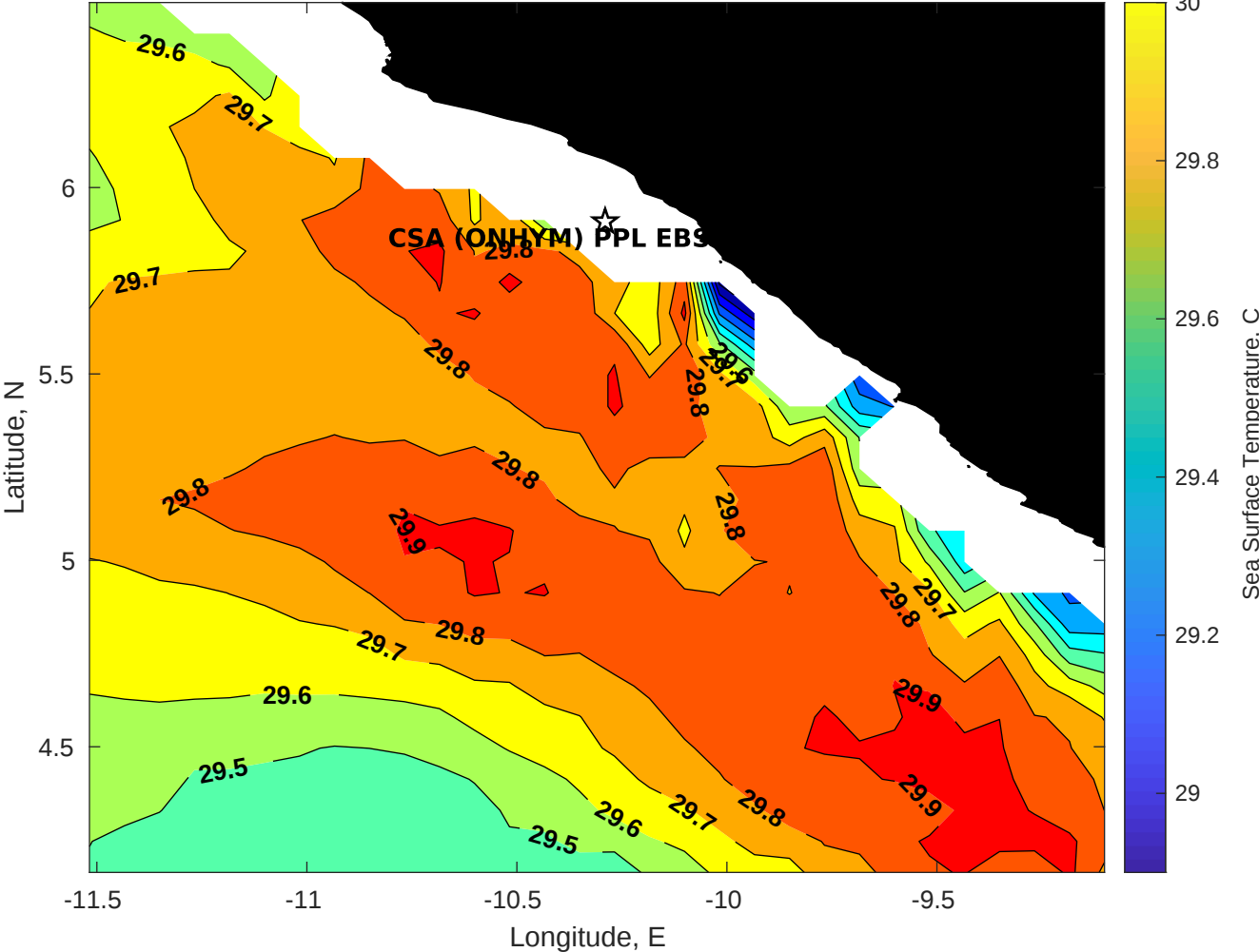
SST for CSA (ONHYM) PPL EBS - Liberia at 25-May-2025 00:00:00
