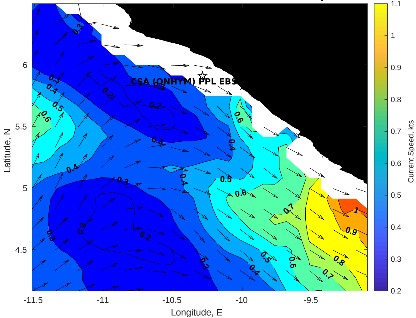
Surface Currents for CSA (ONHYM) PPL EBS - Liberia at 25-May-2025 00:00:00
