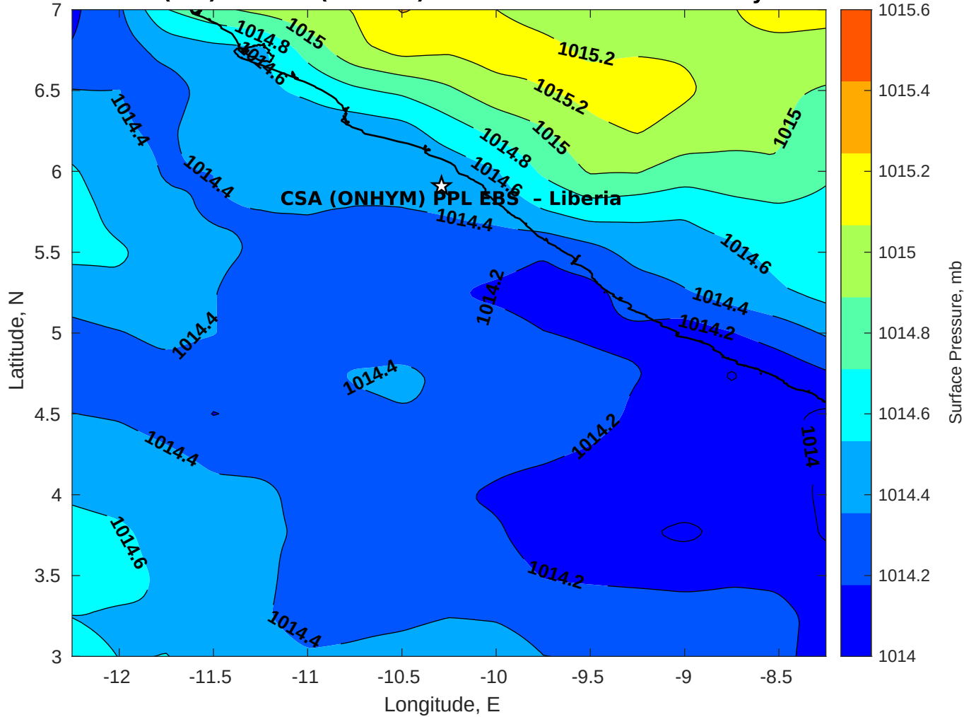
Surface Pressure (mb) for CSA (ONHYM) PPL EBS - Liberia at 26-May-2025 00:00:00
