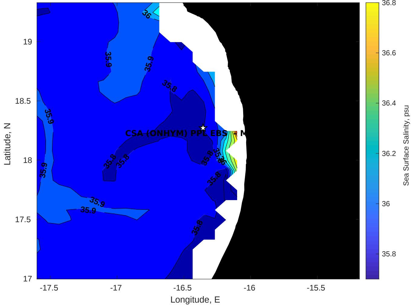
Surface Salinity for CSA (ONHYM) PPL EBS - Mauritania at 25-May-2025 00:00:00
