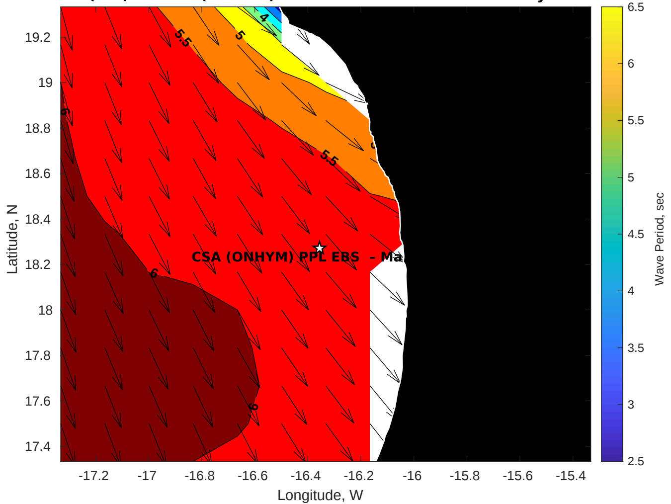
Wave Period (sec) for CSA (ONHYM) PPL EBS - Mauritania at 26-May-2025 09:00:00
