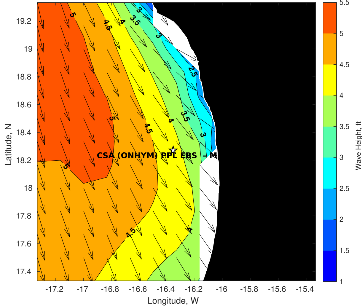
Wave Height (ft) for CSA (ONHYM) PPL EBS - Mauritania at 26-May-2025 09:00:00
