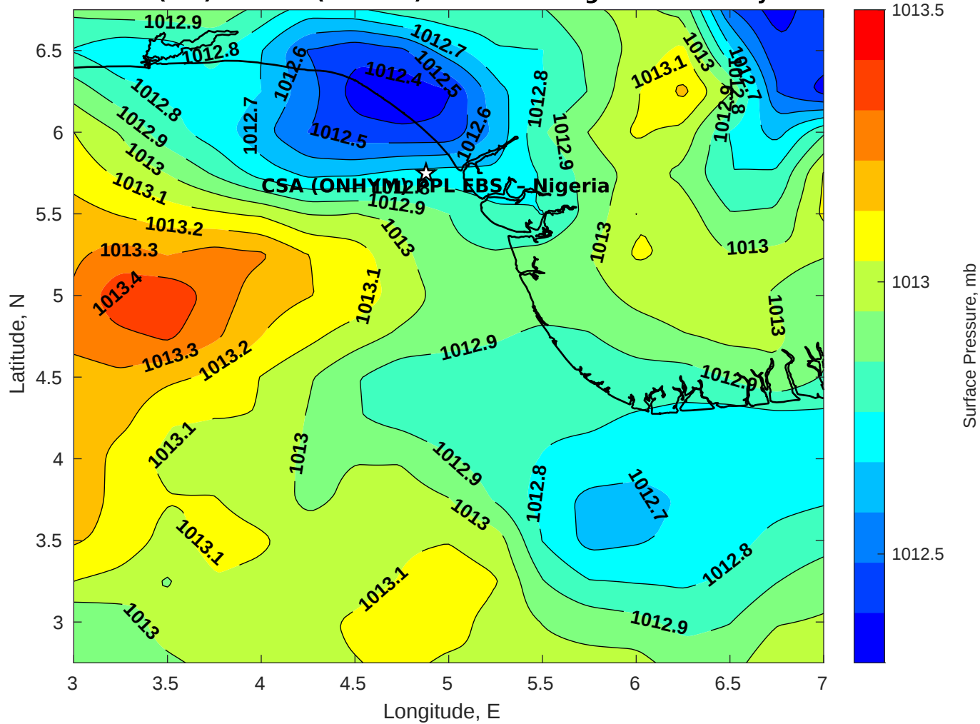
Surface Pressure (mb) for CSA (ONHYM) PPL EBS - Nigeria at 28-May-2025 00:00:00
