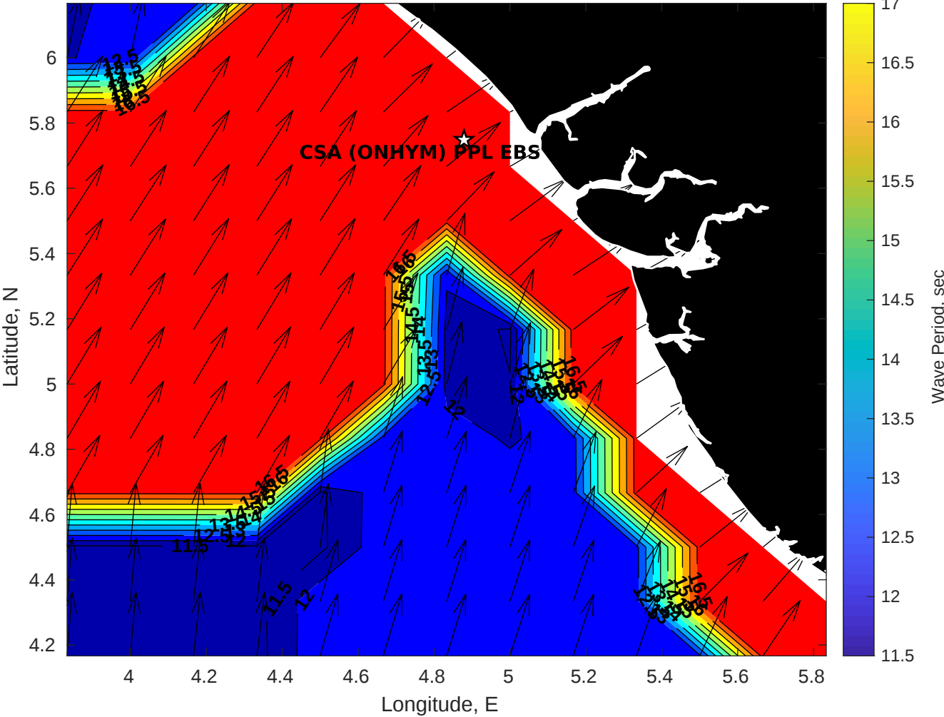
Wave Period (sec) for CSA (ONHYM) PPL EBS - Nigeria at 26-May-2025 09:00:00
