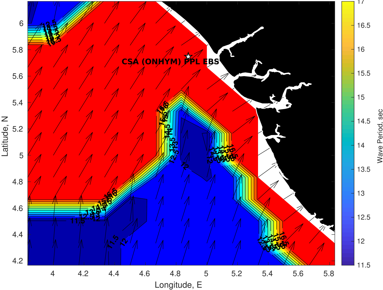
Wave Period (sec) for CSA (ONHYM) PPL EBS - Nigeria at 26-May-2025 09:00:00
