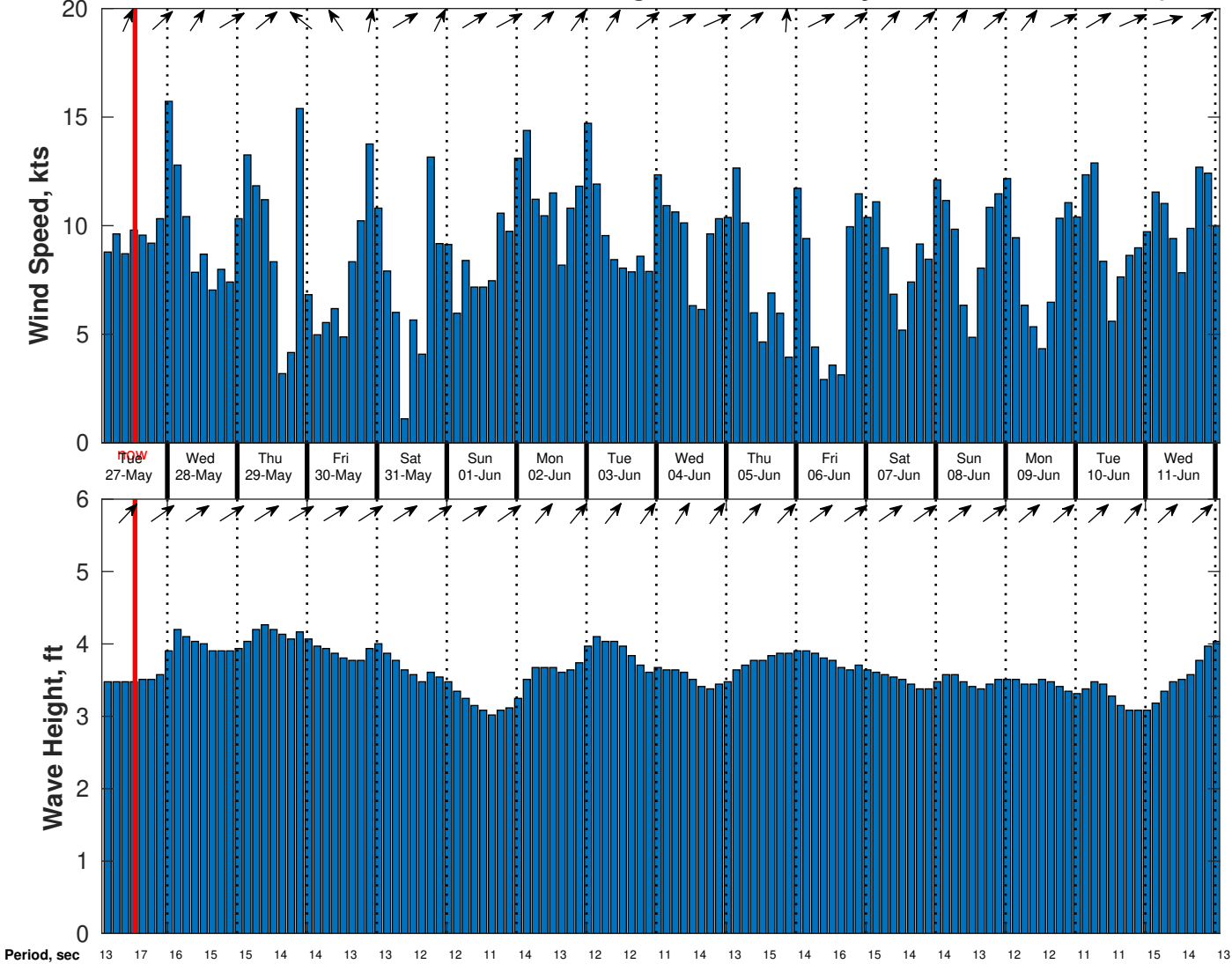
Wind & Wave Forecast for CSA (ONHYM) PPL EBS - Nigeria from 26-May-2025 02:00:00 to 11-Jun-2025 02:00:00
