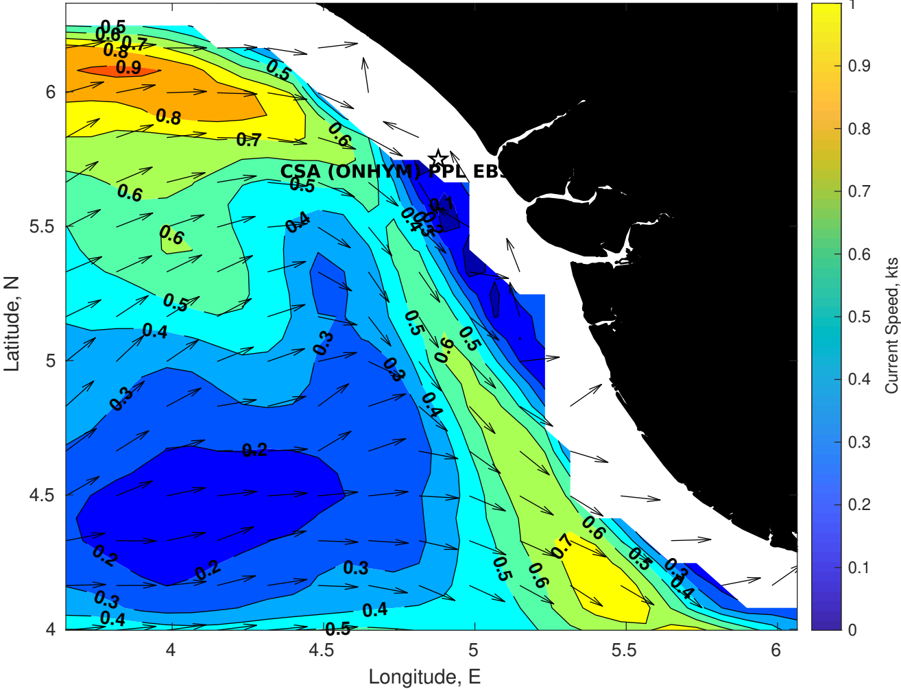
Surface Currents for CSA (ONHYM) PPL EBS - Nigeria at 25-May-2025 00:00:00
