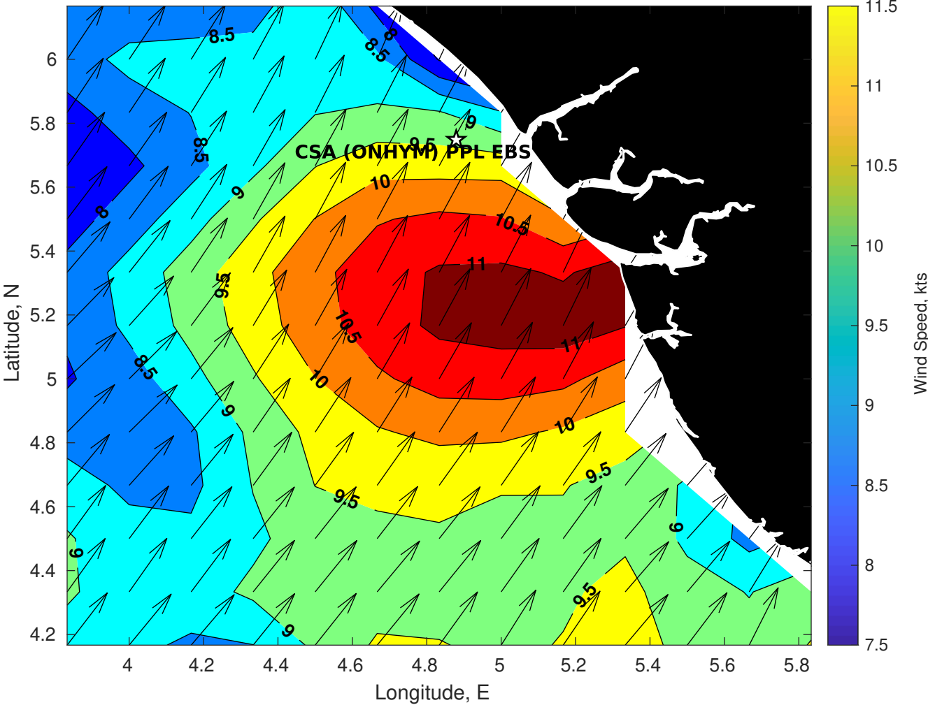
Winds (kts) for CSA (ONHYM) PPL EBS - Nigeria at 26-May-2025 09:00:00
