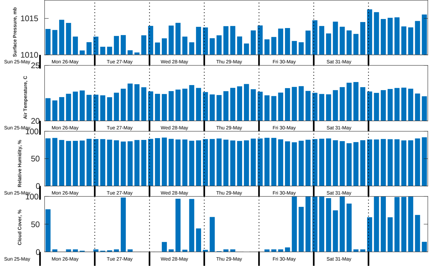
Met Forecast for CSA (ONHYM) PPL EBS - Senegal from 26-May-2025 00:00:00 to 02-Jun-2025 00:00:00
