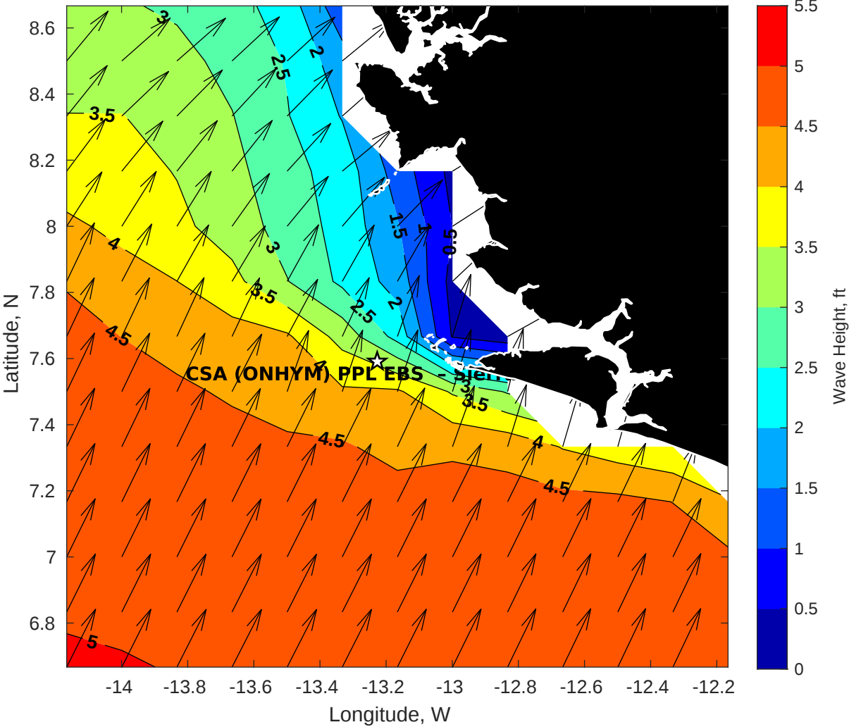
Wave Height (ft) for CSA (ONHYM) PPL EBS - Sierra Leone at 26-May-2025 09:00:00
