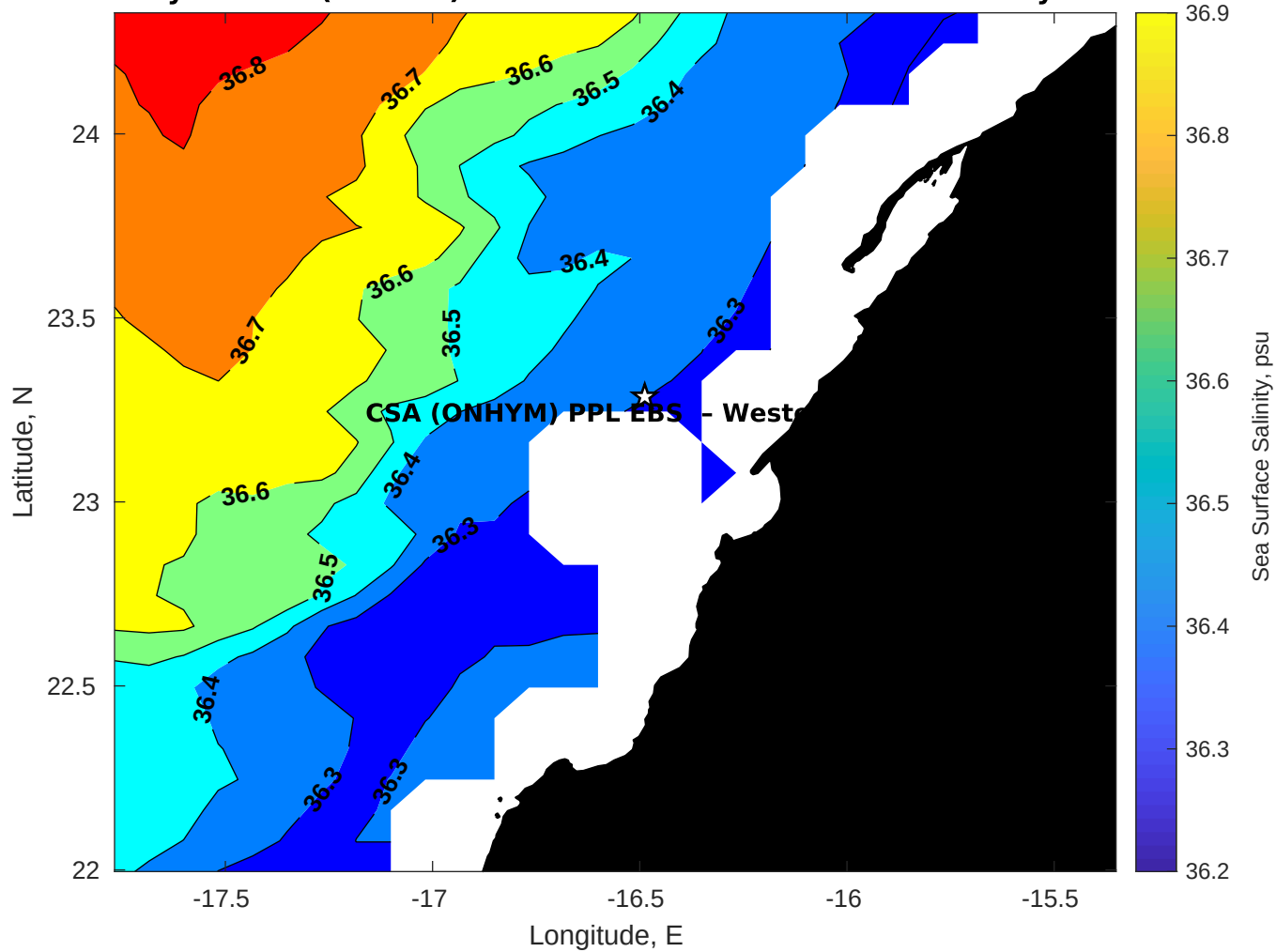
Surface Salinity for CSA (ONHYM) PPL EBS - Western Sahara at 25-May-2025 00:00:00
