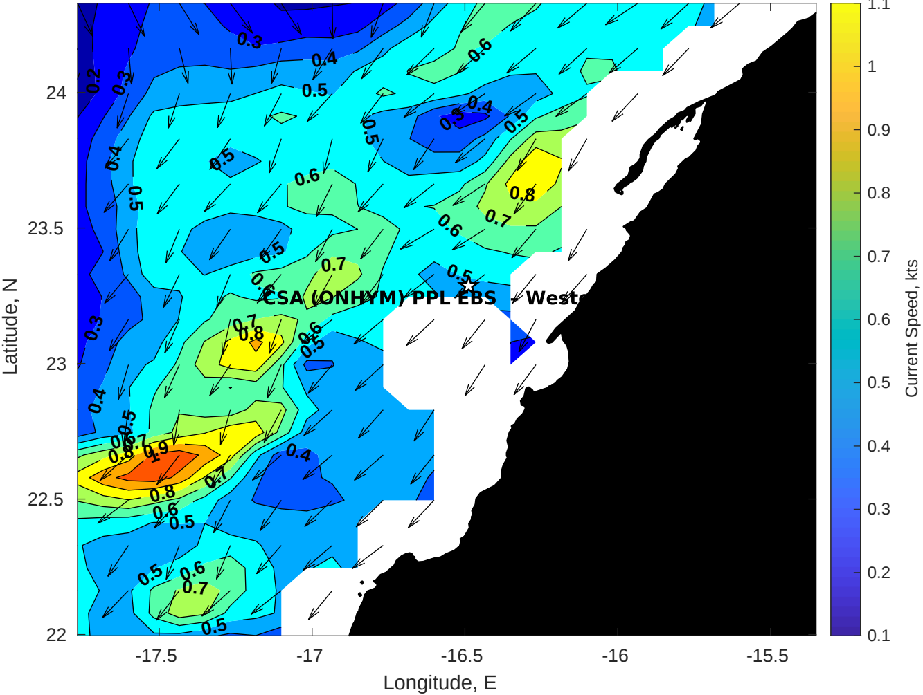
Surface Currents for CSA (ONHYM) PPL EBS - Western Sahara at 25-May-2025 00:00:00
