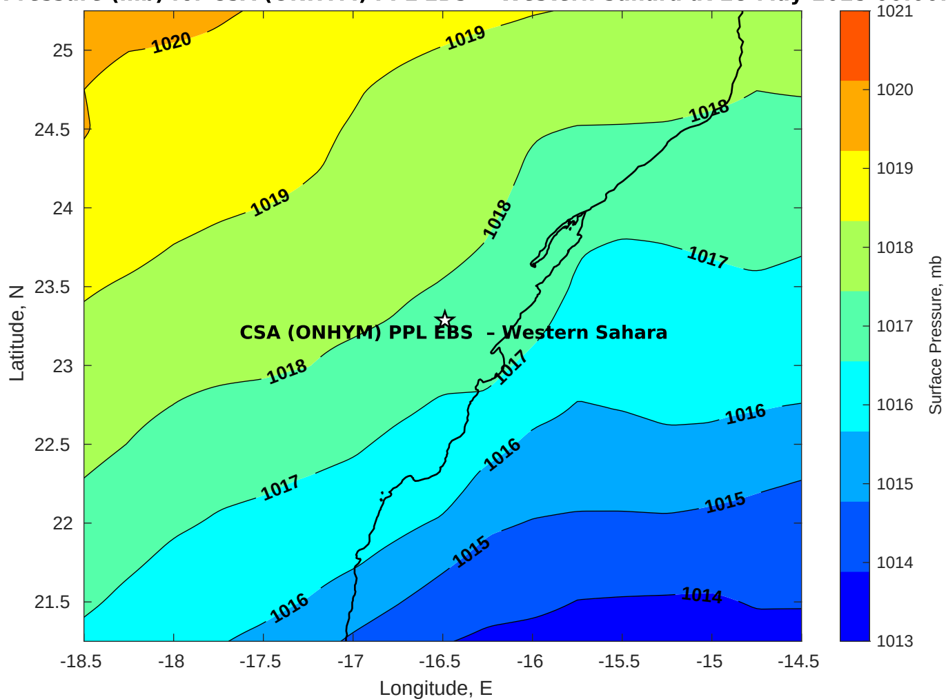
Surface Pressure (mb) for CSA (ONHYM) PPL EBS - Western Sahara at 28-May-2025 00:00:00
