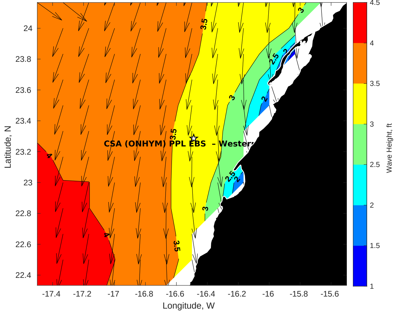
Wave Height (ft) for CSA (ONHYM) PPL EBS - Western Sahara at 26-May-2025 09:00:00
