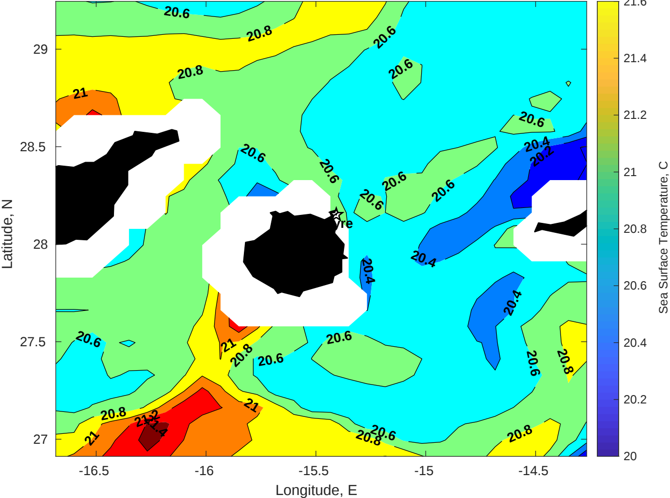
SST for Gyre at 25-May-2025 00:00:00
