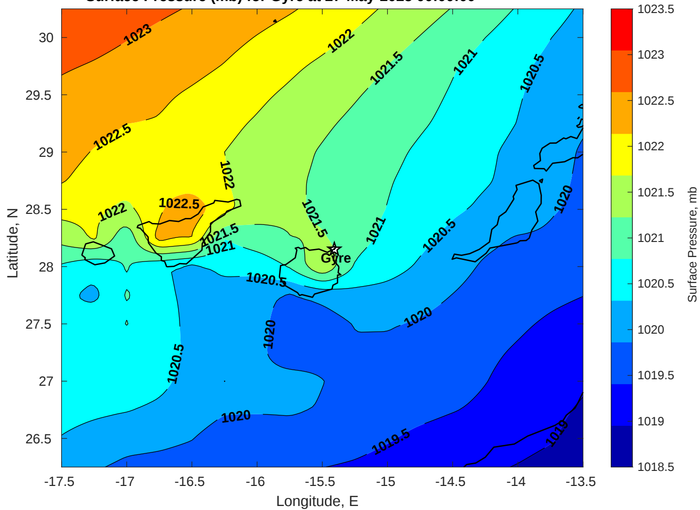
Surface Pressure (mb) for Gyre at 27-May-2025 00:00:00
