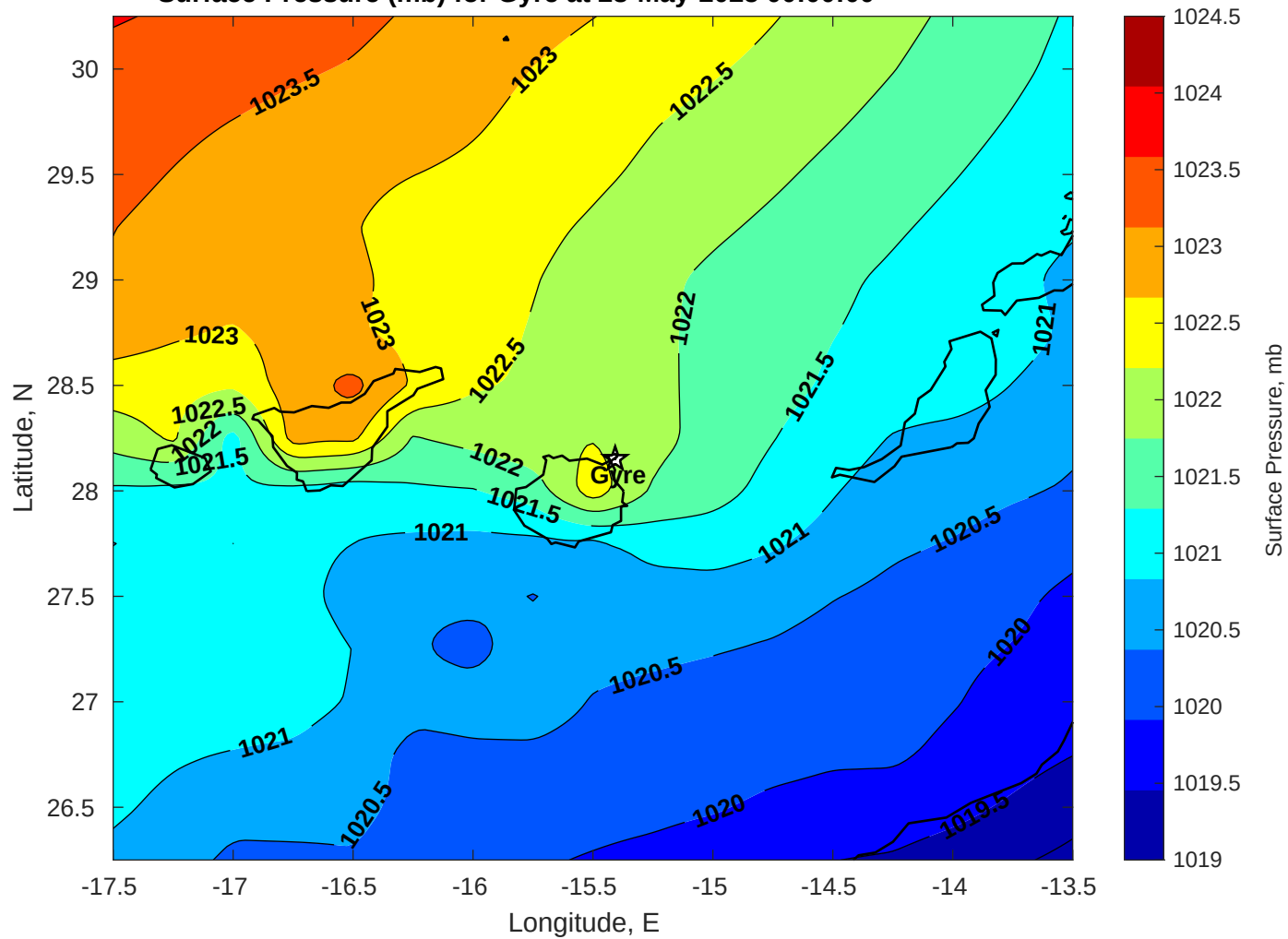
Surface Pressure (mb) for Gyre at 28-May-2025 00:00:00
