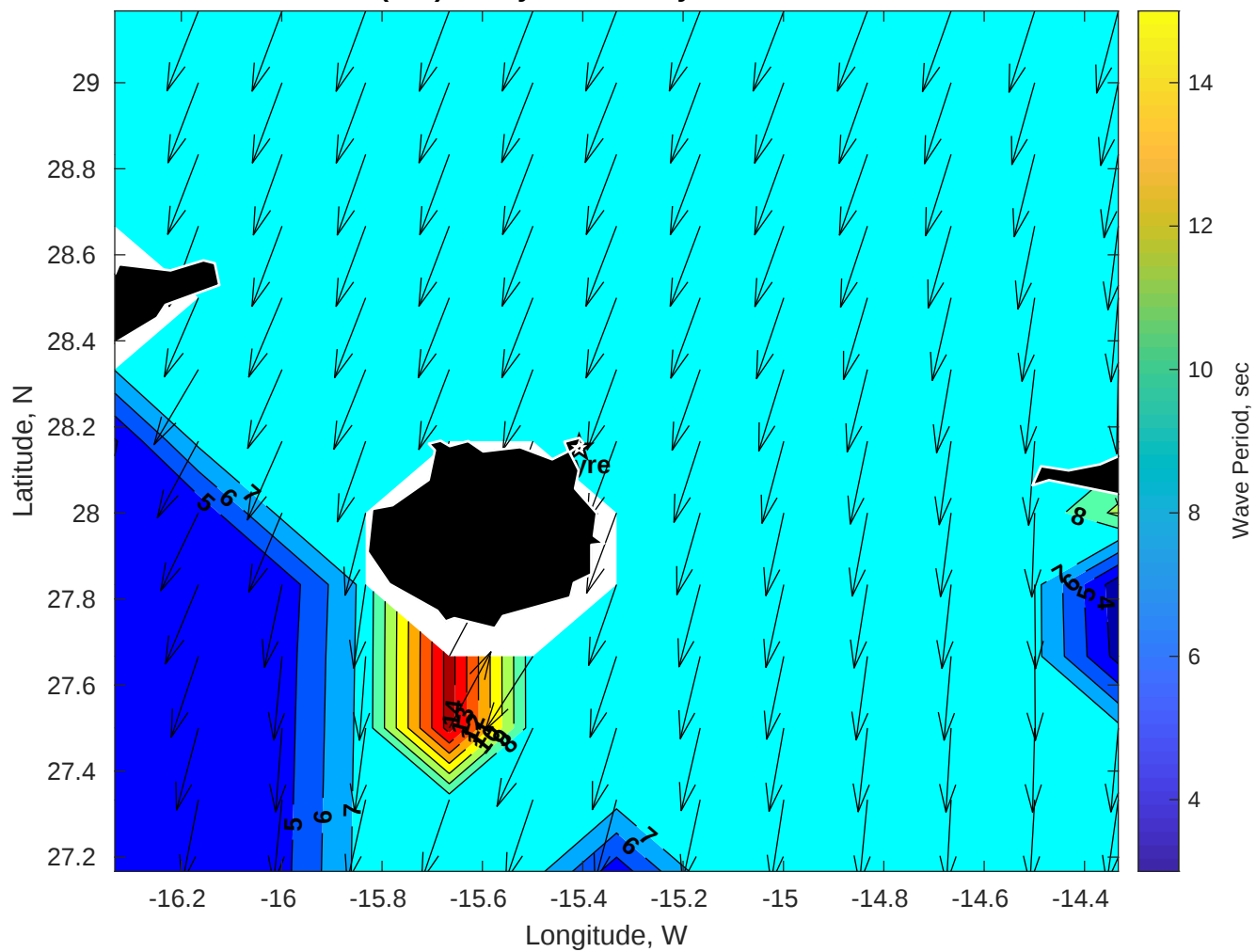
Wave Period (sec) for Gyre at 26-May-2025 09:00:00
