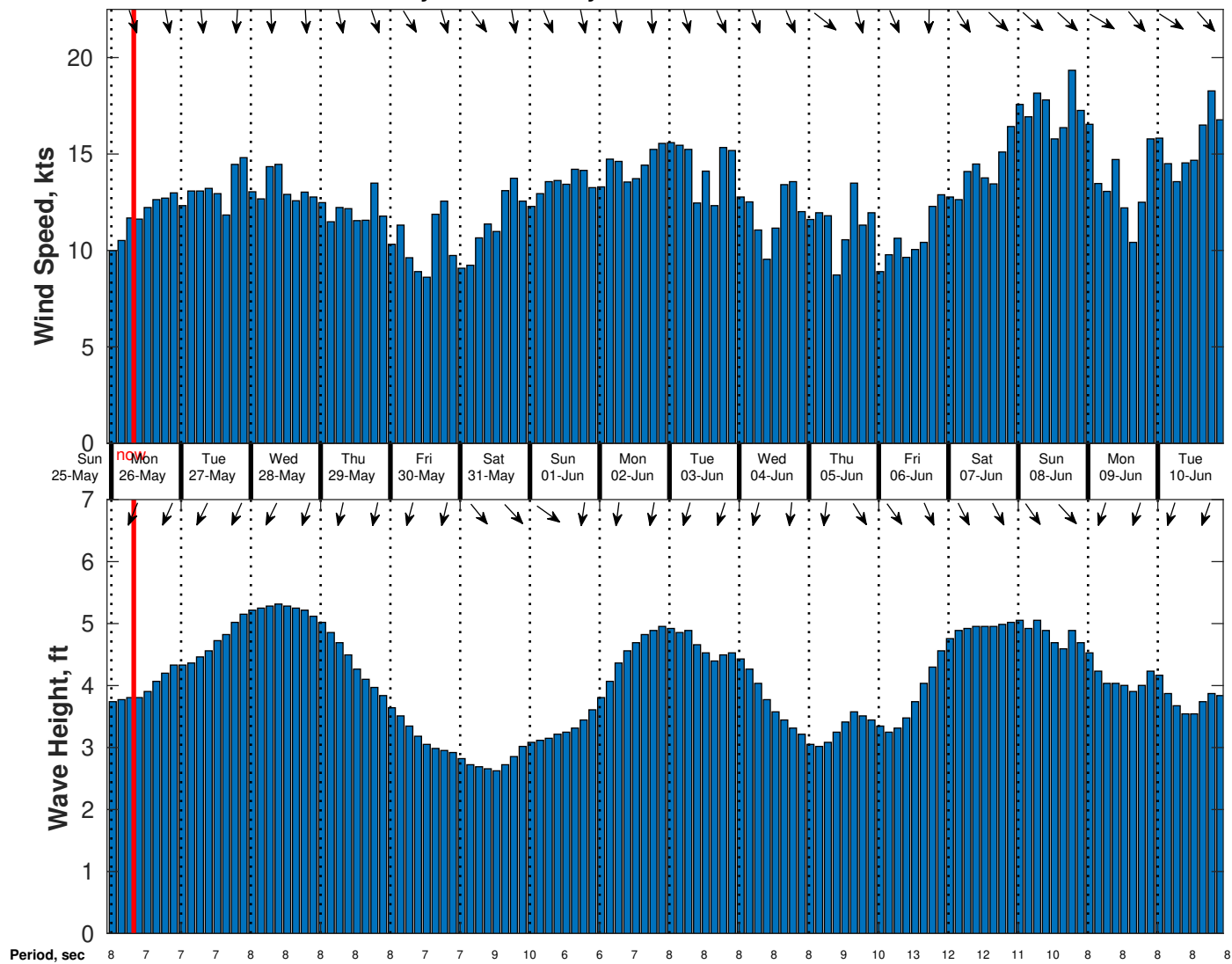
Wind & Wave Forecast for Gyre from 25-May-2025 23:00:00 to 10-Jun-2025 23:00:00
