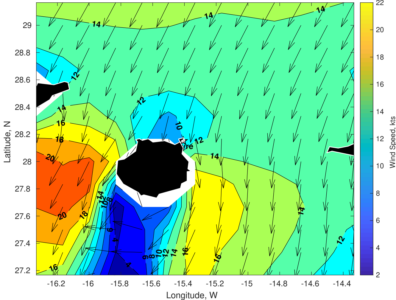
Winds (kts) for Gyre at 26-May-2025 09:00:00
