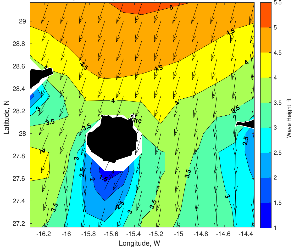
Wave Height (ft) for Gyre at 26-May-2025 09:00:00
