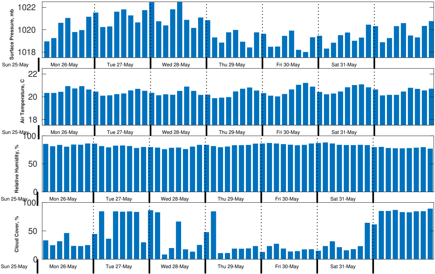
Met Forecast for Gyre from 25-May-2025 23:00:00 to 01-Jun-2025 23:00:00
