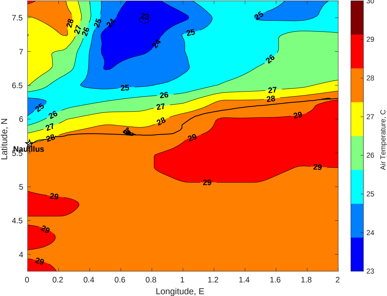
Air Temperature (C) for Nautilus at 26-May-2025
